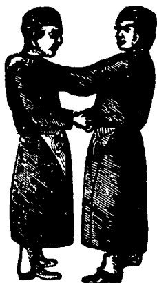
Third Token.
