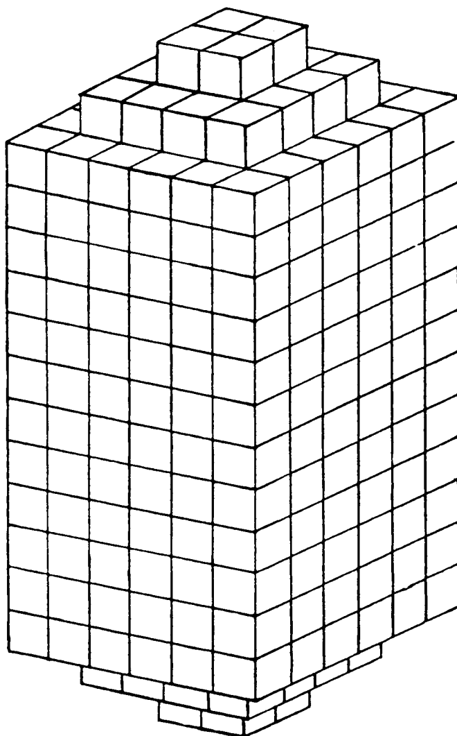
SILVER NITRATE
