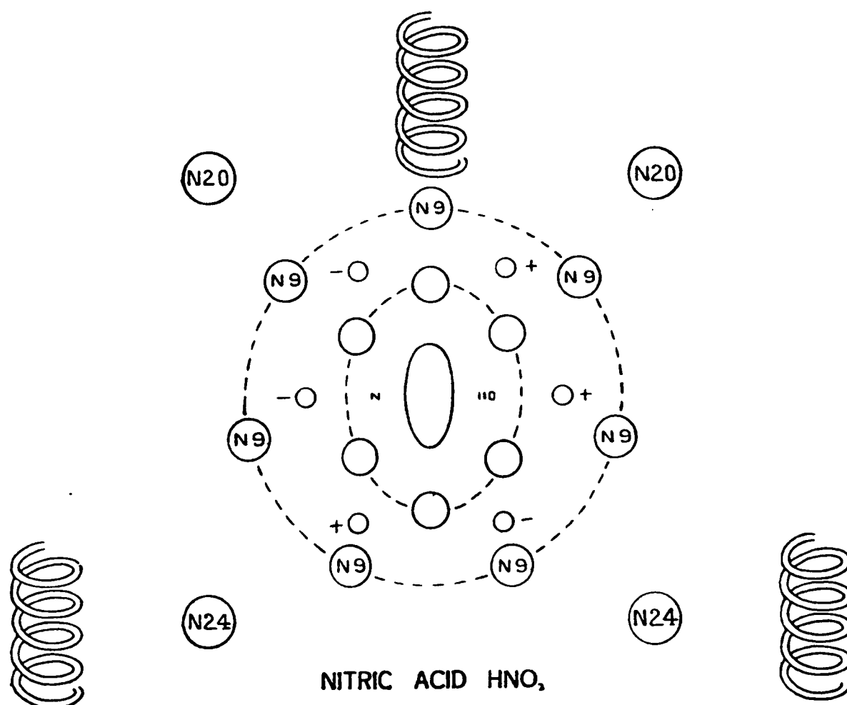
FIG. 186. NITRIC ACID \text{HNO}_3 .
