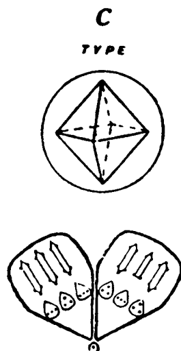
FIG. 191. CARBON
