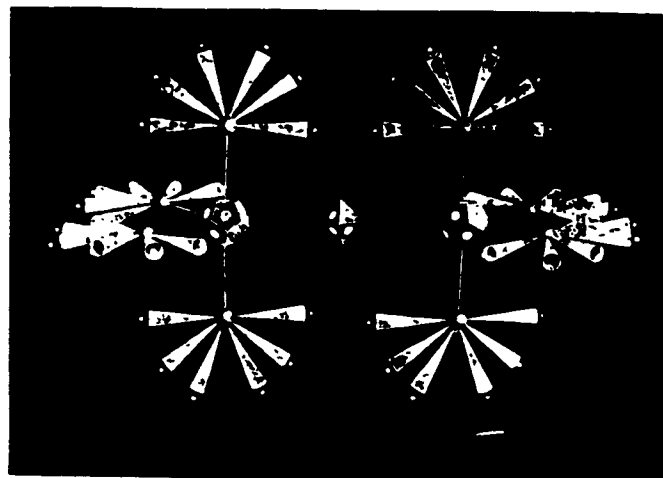
NAPHTHALENE C 10 H 8
