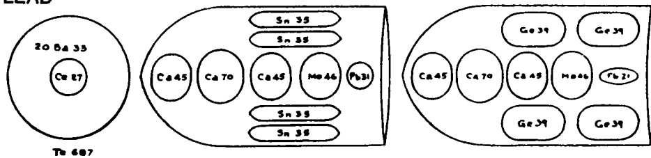
FIG. 139 THE OCTAHEDRON GROUP B
