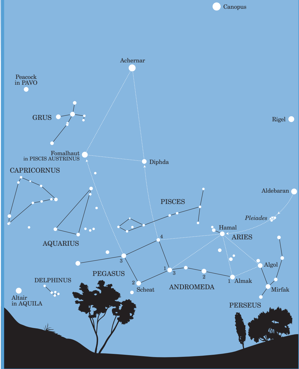
Fig. 36 – Facing North-West – November 10 pm – Horizon for 25° S
