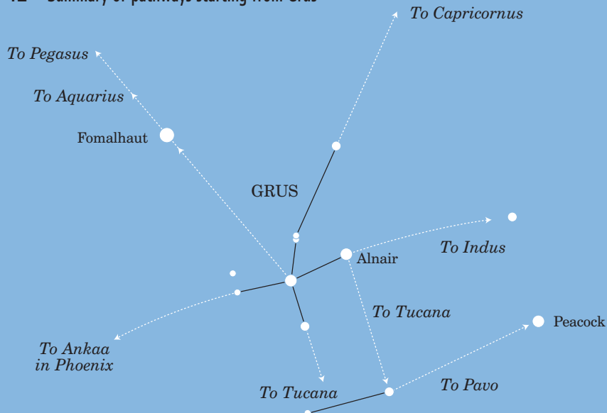
Fig. 42 – Summary of pathways starting from Grus
