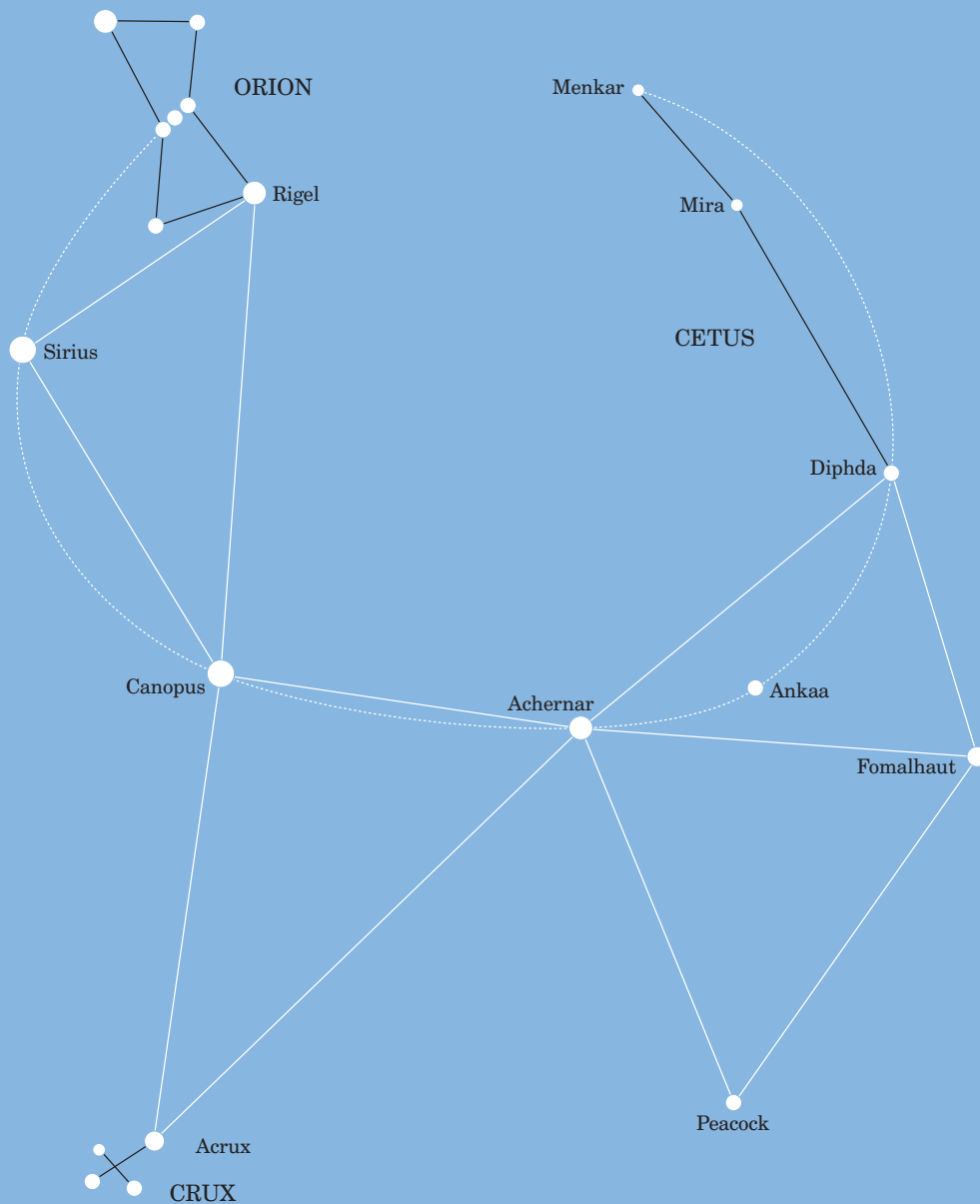
Fig. 48 - Four Major Localizing Triangles
