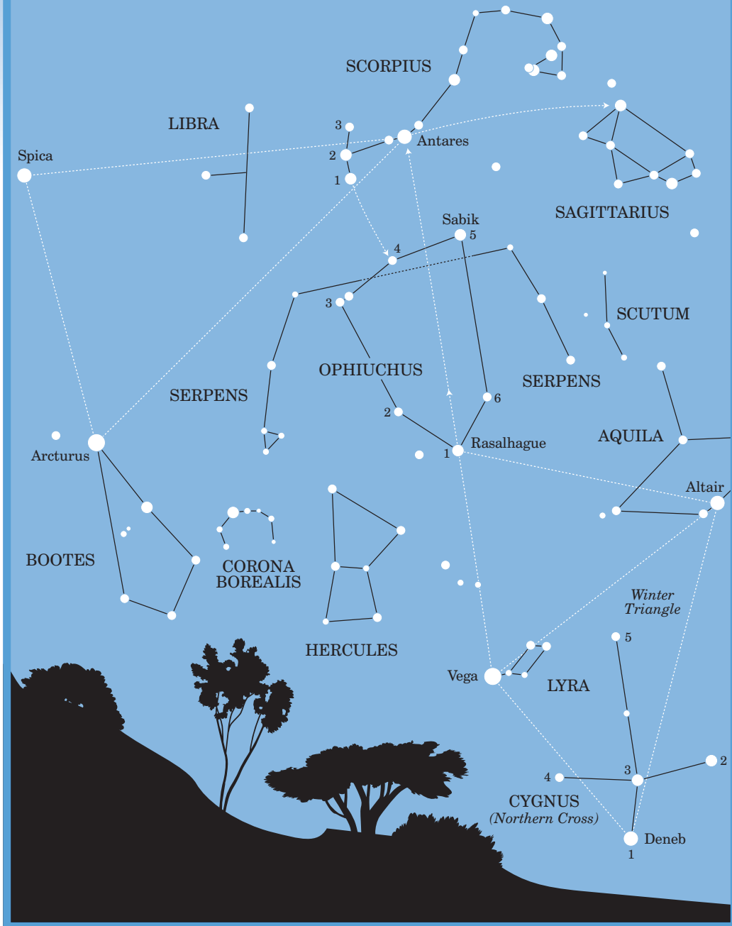
Fig. 40 – Facing North – July 10 pm – Horizon for 25° S
