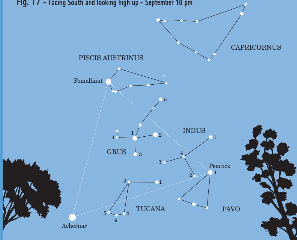
Fig. 17 – Facing South and looking high up – September 10 pm
