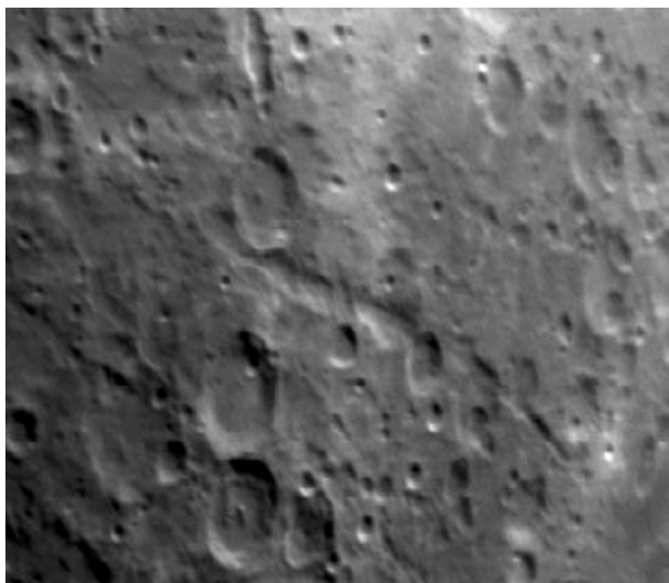
Figure 5.7. Rheita Valley.
