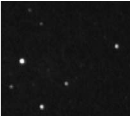
Figure 8.20. NGC 6905: video frame: intensifier. Look carefully near the center.
