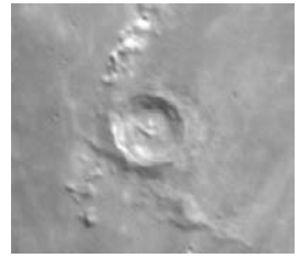
Figure 5.21. a Morning light on Eratosthenes. Note the chains of craterlets below – these are ejecta pits from the formation of nearby Copernicus (just appearing at dawn, bottom center); also note the large lava-filled crater Stadius, center right. b Eratosthenes just 24 hours later.
