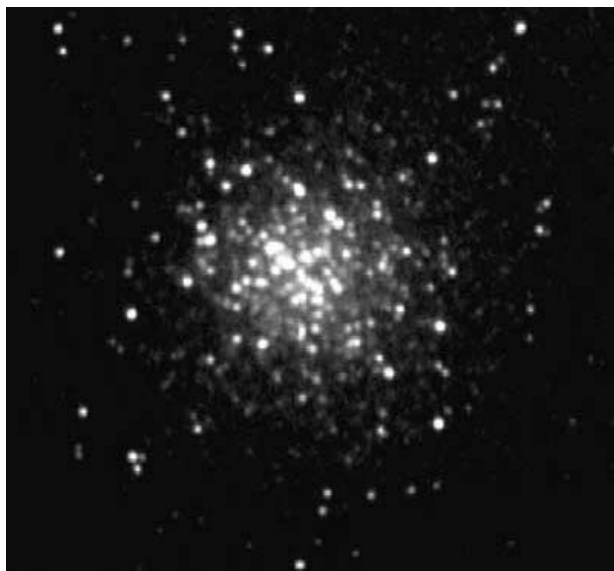
Figure 7.36. NGC 6205 (M13): video frame: intensifier.
