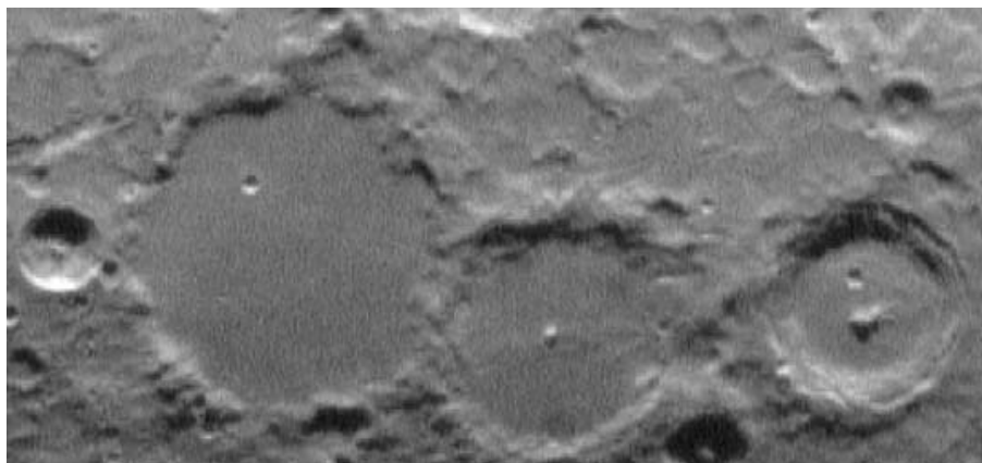
Figure 5.16. Ptolemaeus.
