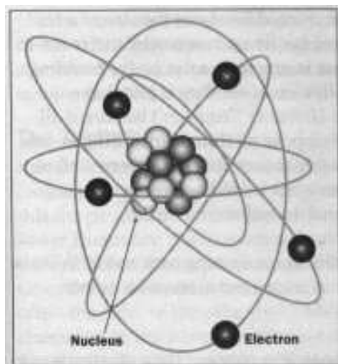
Figure 50: The atoms that make up our 'solid' world are virtually 'empty' to five-sense reality. You could hardly find anything less, 'solid' than an atom. So how can these be the building blocks of the 'solid' physical world? They can't; it's all illusion
