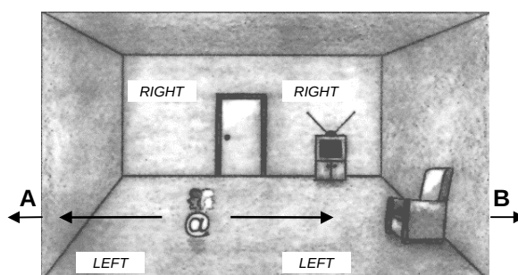
Fig. 35. Vision-reversal problem
