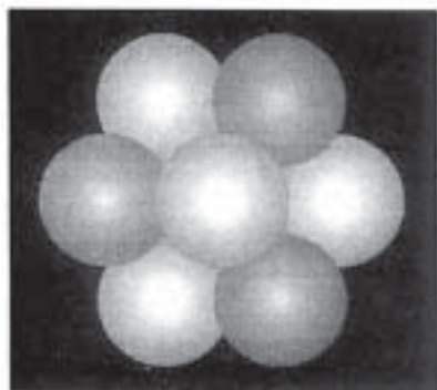
Fig. 6-8. 3D spheres/balls.
