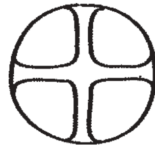
Fig. 2-15. Coptic symbol
