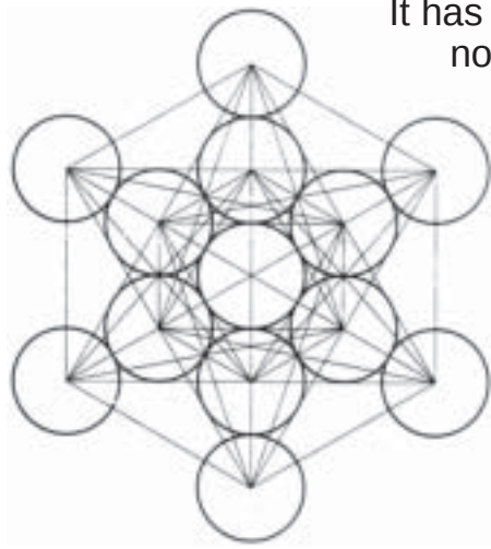
Fig. 6-22. Metatron's Cube.
