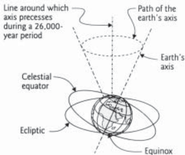
Fig. 2-39. Precession of the equinoxes (the point at which the Earth's celestial equator intersects its ecliptic) is due to the slow rotation of the Earth's axis around a perpendicular to the ecliptic.
