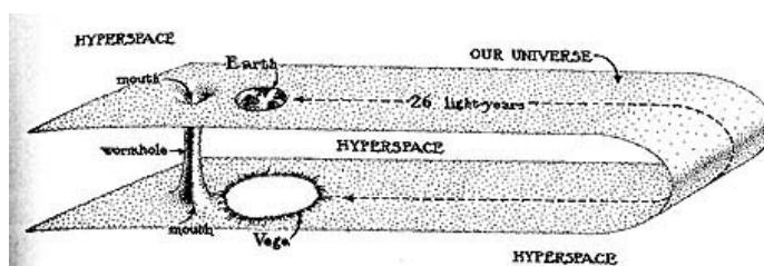
Wormhole illustration on Page 483, Black Holes & Time Warps © 1994 by Kip S. Thorne.
