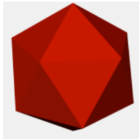
20 equilateral triangle sides of icosahedron.
