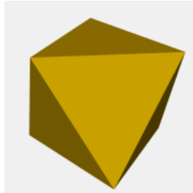
Eight equilateral triangle sides of octahedron.
