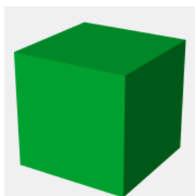
Six sides of cube, or hexahedron.
