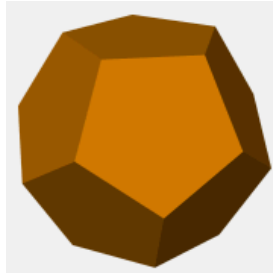
Twelve equilateral pentagon sides of dodecahedron.
