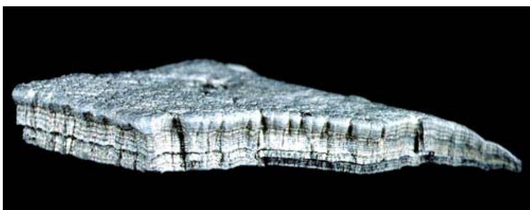
Alleged extraterrestrial metal taken from the bottom of a "wedge-shaped craft in 1947" was created from alternating layers of 1-4 microns dark bismuth and 100-200 microns silver magnesium/zinc alloy, approximately twenty-five to thirty layers thick. Each of six pieces received were "formed" with a curvature that tapered, as shown to the right in photo magnification above.
