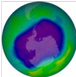
From September 21-30, 2006, the average area of the ozone hole was the largest ever observed, at 10.6 million square miles (27.5 million square kilometers). The blue and purple colors are where there is the least ozone (loss of 40 million tons of ozone), and the greens, yellows, and reds are where there is more ozone. Image courtesy NASA.
