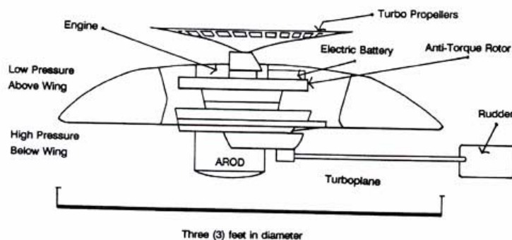
Airborne Remotely Operated Device, AROD THE RPV
