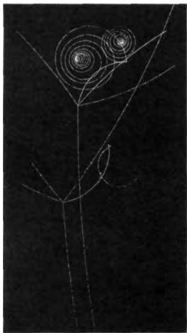
Subatomic particle tracks from the 'bubble chamber'. Particles which are not 'things' but rather packets or foci of energy, collide and create these beautiful patterns. The physicist Fritjof Capra rightly sees in this a parallel to the Indian dance of Shiva, which represents the mystical creation. From the point of view of Pythagorean number theory, it is interesting to note the formation at this fundamental state of spirals and the division into four, the 'number' of principal matter.
