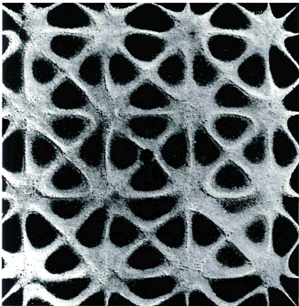
37 A sonorous figure, also produced by piezo-electric excitation. Square steel plate 23x23 cm, thickness 1 mm. Frequency 6700 cps. In such experiments as these, the formation of nodal lines of sand can be accurately observed. They often pile up like dunes.
