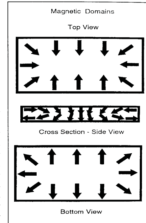
Figure 3. Magnetic domain alignment in barium ferrite after conditioning.
