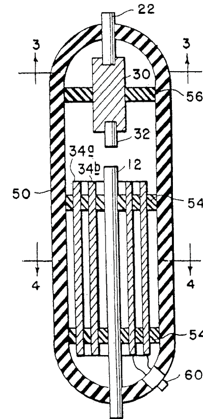
Figure 1 Gray's scalar compression tube from U.S. Patent 4,661,747. The hollow cathode 34 (a & b) contains negatively charged glow plasma. A sharp, unipolar spark from anode 12 to 32 triggers avalanche breakdown in the cylindrical gap between cathode 34 and anode 12 resulting in a symmetrical, imploding ionization shock wave originating from the glow plasma. The ionization wave front propagates downward in the cylindrical gap to launch a negative, vacuum polarization transient out the bottom of the tube guided on electrode 12.
