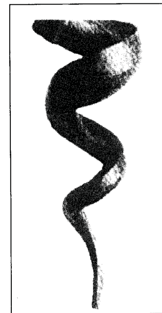
Figure 2. Schauburger's implosion vortex pipe.
