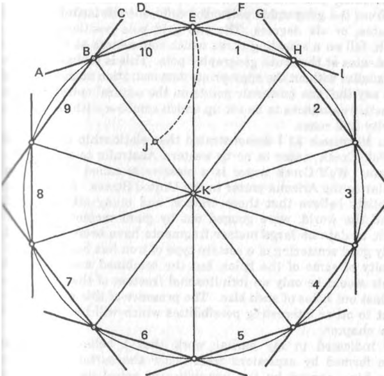
DIAGRAM THE HARMONICS OF A DECAGON
