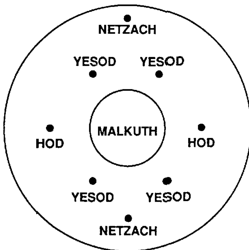
Fig. 23. Southern Hemisphere / Heavens
