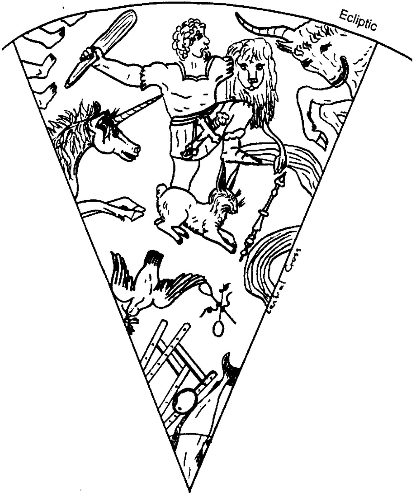
Ecliptic South Pole Figure 31
