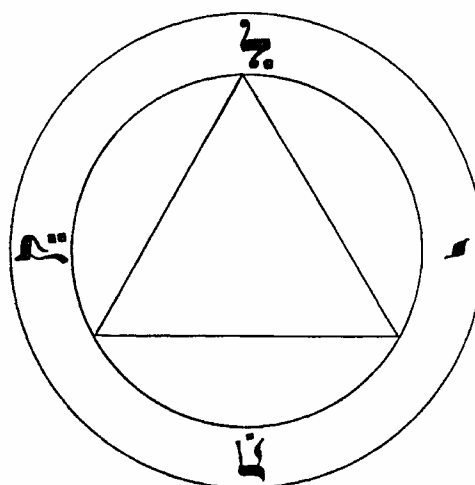
Fig. 15. Little complementary circle.
