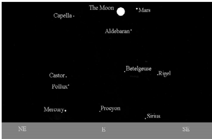
Looking low above the eastern horizon before sunrise on August 7, 2007.
