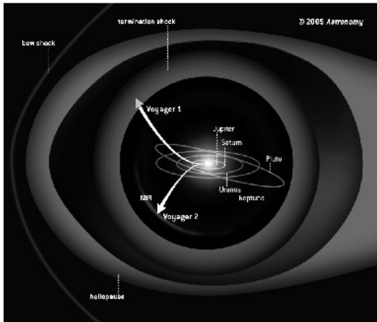
NASA's ring of hydrogen particles.
