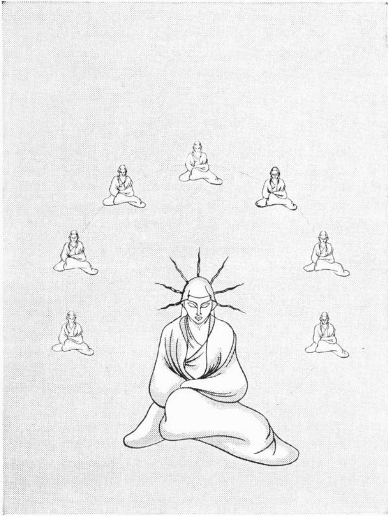
THE SEVEN PRIMARY LAWS OR MOTIONS OF TAO. Emanated as modes of the transcendental being, realization establishes the foundations or polarities of reality within itself.
