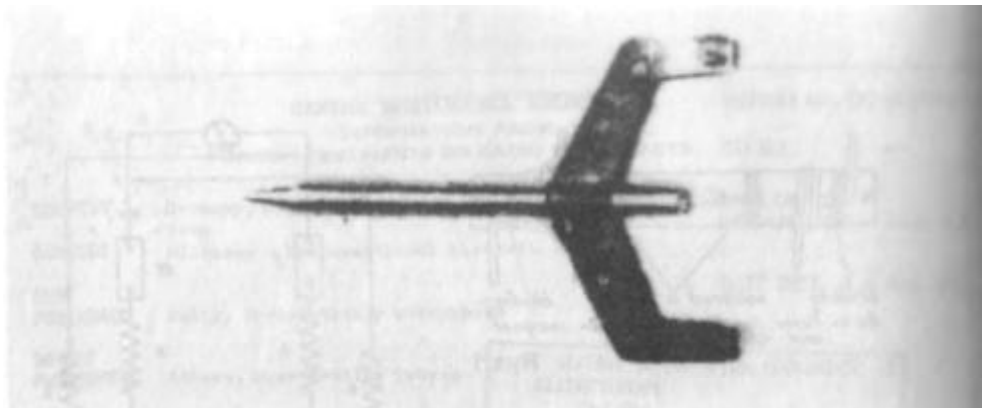
Above: Wave guide used in electromagnetic experiments at Peenemünde.
