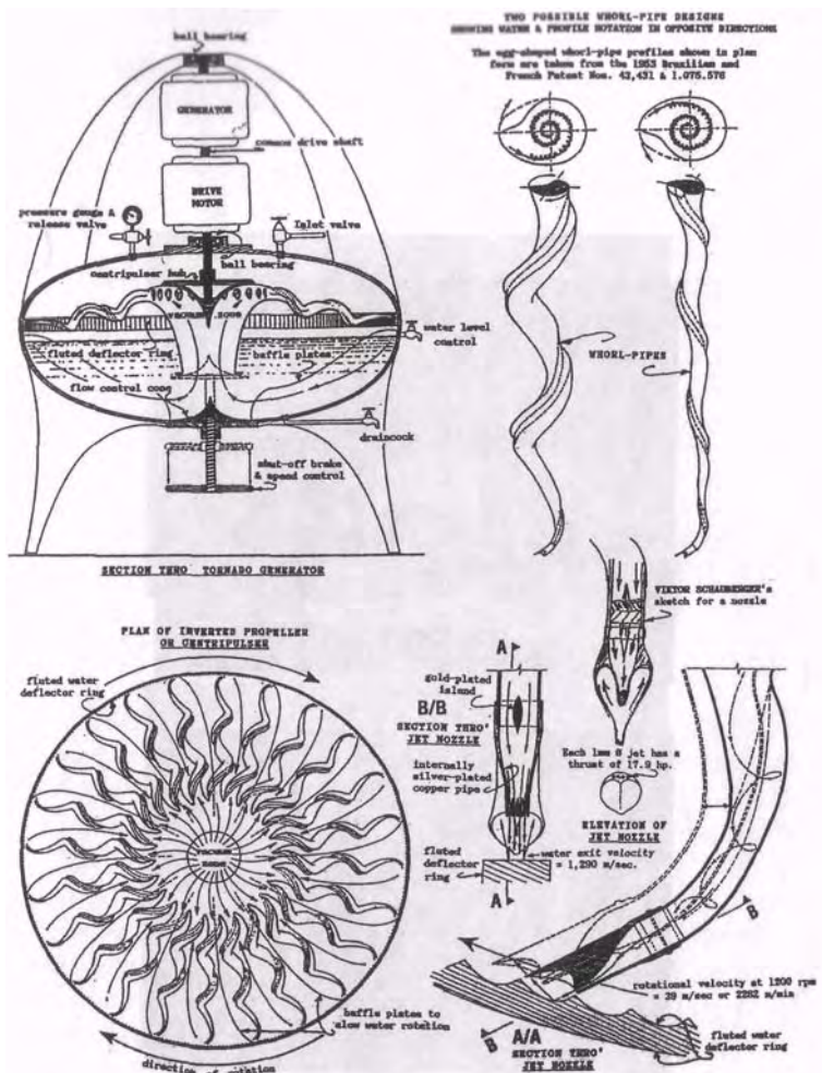
Schauberg's Postwar "Tornado" Generator
