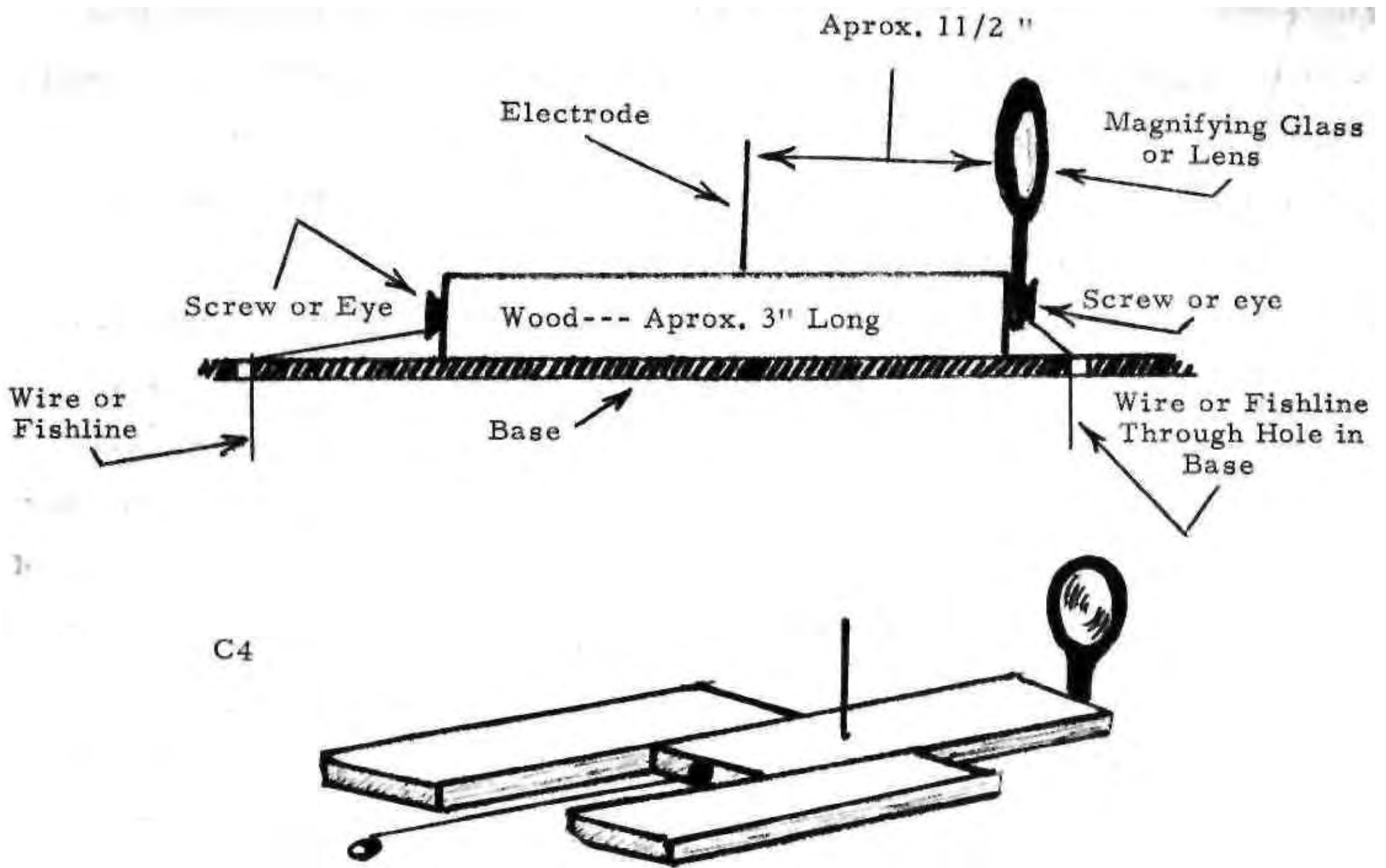
Focusing Assembly Mounted on Base
