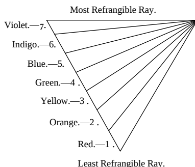
Fig. 33. PRISMATIC SPECTRUM.
