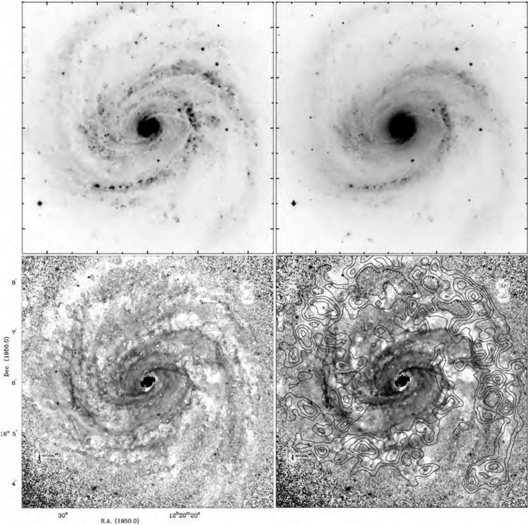
Fig. 5.26. Sbc galaxy M100: 26'' = 2 \text{ kpc} . Top, B band (left) and I band (right); in these negative images, dark dust lanes just inside the bright spiral arms appear as thin light filaments. Lower panels show B - K color. Light areas are blue with young massive stars, and dark regions show red regions where dust lanes spiral into the galaxy center; the overexposed core appears as a dark hole. Contours show H\alpha emission (left) and H\text{I} gas (right), which are both concentrated in spiral arms; the center is largely empty of H\text{I} – J. Knapen 1996 MNRAS 283 , 251.
