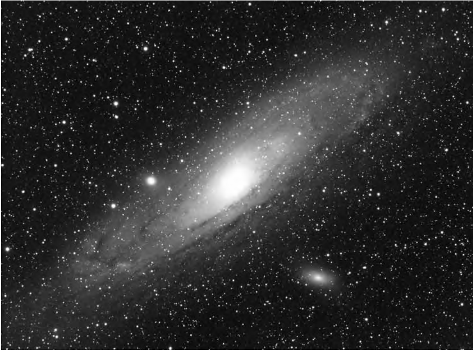
Fig. I.14. Our nearest large neighbor, the Andromeda galaxy M31; north is to the right, east is upward. Note the large central bulge of this Sb galaxy, and dusty spiral arms in the disk. Two satellites are visible: M32 is round and closer to the center, NGC 205 is the elongated object to the west – O. Nielsen.
