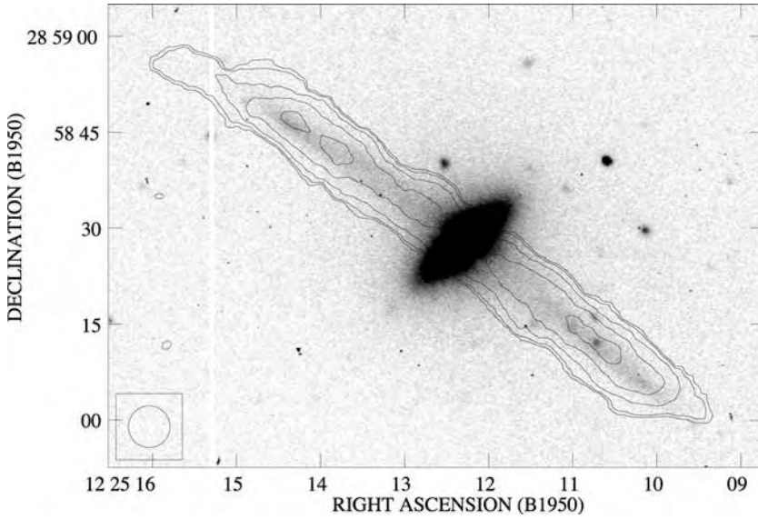
Fig. 5.17. A negative image of the S0 galaxy UGC 7576 in the V band: a thin ring of dust, gas, and stars orbits over the galaxy's pole. Contours show 5 \times 10^9 M_\odot of HI gas in the polar ring; the disk of the S0 galaxy has hardly any cool gas. The circle on the left shows the radio telescope's beam – A. Cox.
