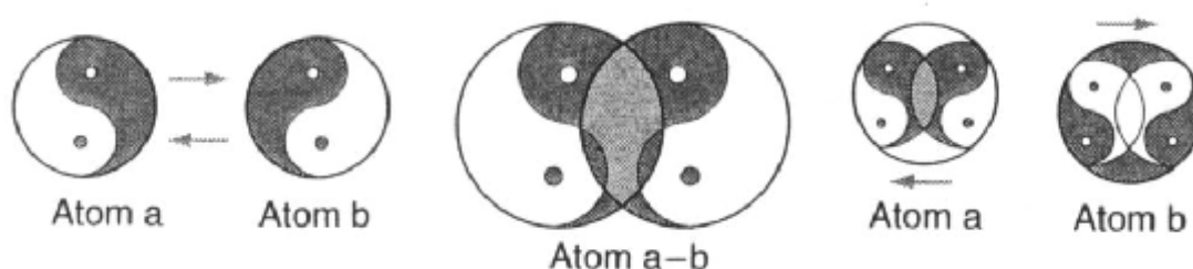
Fig 21: Atomic mitosis, or 'symmetry': the entanglement process
