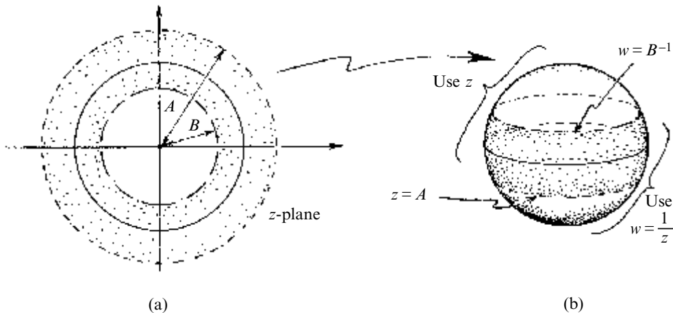
Fig. 9.5 (a) The annulus of convergence for a Laurent series F(z) = F^+ + \alpha_0 + F^- , where F^+ = \cdots + \alpha_{-2}z^{-2} + \alpha_{-1}z^{-1} , F^- = \alpha_1z^1 + \alpha_2z^2 + \cdots . The radius of convergence for F^+ is A and, in terms of w = z^{-1} , for F^- is B^{-1} . (b) The same, on the Riemann sphere (see Fig. 8.7), where z refers to the extended northern hemisphere and w (= z^{-1}) to the extended southern hemisphere.
