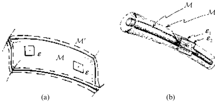
Fig. 31.2 Geometrical description of supersymmetry generators. (a) For a single generator \varepsilon , regard our n -manifold \mathcal{M} as a hypersurface in an (n + 1) -manifold \mathcal{M}' , where \varepsilon is a 1-form in \mathcal{M}' defined at \mathcal{M} (and \varepsilon defines the n -plane tangent to \mathcal{M} as in Fig. 12.7, §12.3). We are interested in \mathcal{M}' , only to ‘first order’ at \mathcal{M} , but \mathcal{M}' supplies an additional dimension pointing away from \mathcal{M} . (b) With N supersymmetry generators \varepsilon_1, \dots, \varepsilon_N , the n -manifold \mathcal{M} is now regarded as a submanifold of an (n + N) -manifold \mathcal{M}' , where again we are interested in \mathcal{M}' only to first order away from \mathcal{M} . The N independent 1-forms \varepsilon_1, \dots, \varepsilon_N ‘feel out’ the N extra directions pointing out from \mathcal{M} , and into \mathcal{M}' .
