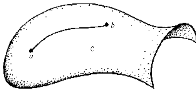
Fig. 20.3 Hamilton's principle. The Euler–Lagrange equations tell us that the motion of Q through \mathcal{C} is such as to make the action—the integral of \mathcal{L} along a curve, taken between two fixed points a, b , in \mathcal{C} —stationary under variations of the curve.
