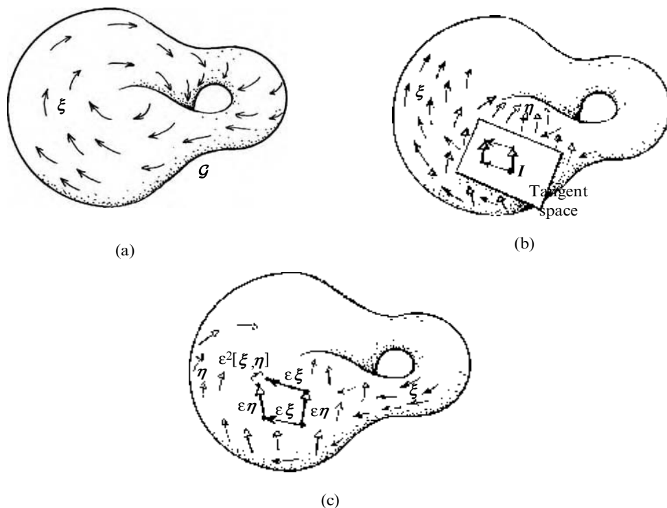
Fig. 14.15 Lie algebra operations, interpreted geometrically in the continuous group manifold \mathcal{G} . (a) Pre-multiplication of each element of \mathcal{G} by an infinitesimal group element \xi (Lie algebra element) gives an infinitesimal shift of \mathcal{G} , i.e. a vector field \xi on \mathcal{G} . (b) To first order, the product of two such infinitesimal motions \xi and \eta just gives \xi + \eta , reflecting merely the structure of the tangent space (at I ). (c) The local group structure appears at second order, \epsilon^2[\xi, \eta] , providing the O(\epsilon^2) gap in the ‘parallelogram’ with alternate sides \epsilon\xi and \epsilon\eta at I .
