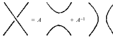
Fig. 32.8 The basic algebraic identity for the Kauffman algebra is illustrated, where q = A^2 = e^{i\pi/r} , giving a q -deformed version of the ‘binor’ algebra underlying spin-network theory (for which A = -1 , and the crossing issues of Fig. 32.7 do not occur).
