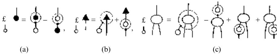
Fig. 14.17 Diagrams for Lie derivative (a) of a vector \eta : (\mathfrak{L}_\xi \eta)^a = \xi^a \nabla_a \eta^b - \eta^a \nabla_a \xi^b ; (b) of a covector \alpha : (\mathfrak{L}_\xi \alpha)_a = \xi^b \nabla_b \alpha_a + \alpha_b \nabla_a \xi^b ; and (c) of a [2] -valent tensor Q : \mathfrak{L}_\xi Q_{ab}^c = \xi^u \nabla_u Q_{ab}^c + Q_{ub}^c \nabla_a \xi^u + Q_{au}^c \nabla_b \xi^u - Q_{ab}^u \nabla_u \xi^c .
