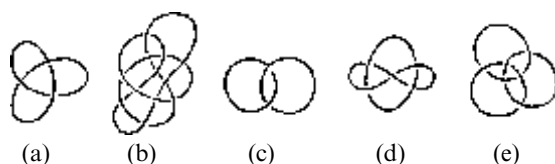
Fig. 32.6 Knots and links. (a) A trefoil knot—an example of a knotted loop. (b) An example of a (non-obviously, to the eye) unknotted loop. (c) A simple link between two loops. (d) A Whitehead link, where the two loops cannot be separated though they have zero ‘linking number’ (the net number of times each meets a surface spanning the other) (e) Borromean rings, which cannot be separated, despite no pair of them being linked.
