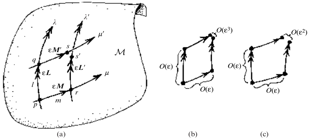
Fig. 14.9 (a) Try to make parallelogram out of geodesics. Take two geodesics \lambda, \mu , through p , in \mathcal{M} , with respective tangent vectors L, M at p and corresponding affine parameters l, m . Take q an affine distance l = \varepsilon along \lambda from p , and r an affine distance m = \varepsilon along \mu from p (with \varepsilon > 0 a fixed small number). The geodesic segments pq and pr have respective ‘arrow-lengths’ \varepsilon L, \varepsilon M . To make the parallelogram, move M from p to q along \lambda by parallel transport ( \nabla_L M = 0 along \lambda ) giving us a neighbouring geodesic \mu' to \mu , extending from q to s along \mu' by an affine distance \varepsilon along the new ‘parallel’ arrow \varepsilon M' . Similarly, move L from p to r by parallel transport along \mu , and extend from r to s' by a parallel arrow \varepsilon L' measured out from q an affine distance m = \varepsilon along \lambda' . (b) Generally s \neq s' and the parallelogram fails to close exactly, but this gap is only O(\varepsilon^3) if the torsion \tau vanishes. (c) If there is a non-zero torsion \tau , this will show up as an O(\varepsilon^2) term.
