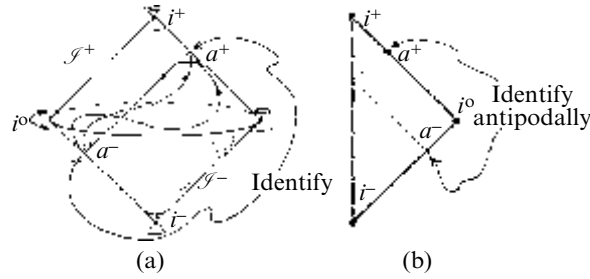
Fig. 33.9 Compactified Minkowski space \mathbb{M}^\# is obtained from ordinary Minkowski space \mathbb{M} by adjoining its future and past null infinities \mathcal{J}^+ and \mathcal{J}^- and then identifying them appropriately as \mathcal{S} . (a) The future light cone of any point a^- on \mathcal{J}^- focuses back to another vertex a^+ on \mathcal{J}^+ (this ‘light cone’ being, in ordinary terms, simply the history of a plane wavefront travelling at the speed of light), and a^- is to be identified with a^+ . Spacelike infinity i^0 and the past and future timelike infinities i^- and i^+ are all to be identified as a single point i . (b) This identification \mathcal{S} is shown, in terms of the strict conformal diagram of Fig. 27.16b, where a^- is antipodal to a^+ on the ‘ S^2 of rotation’ for the whole diagram.
