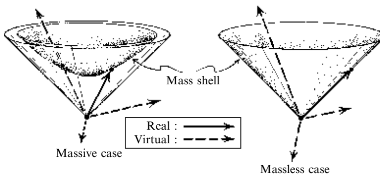
Fig. 26.6 The mass shell in momentum space. (Compare Figs. 18.7, 18.17.) For real (free) particles of rest-mass M , the 4-momentum p^a lies on the mass shell (so p^a is future timelike or future null with p_a p^a = M^2 ), but virtual particles, in the interior of a Feynman graph, can be ‘off shell’.
