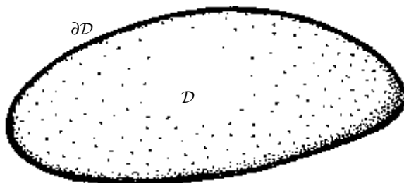
Fig. 20.10 If desired, we may regard the \mathcal{A} and \mathcal{B} of Fig. 20.9 to be joined together—but taken with opposite orientations (see Fig. 12.16)—so as to constitute the boundary \partial\mathcal{D} of a (compact) spacetime 4-volume \mathcal{D} . Hamilton's principle (Fig. 20.3) expresses the stationarity of \int_{\mathcal{D}} \mathcal{L}\epsilon for a given field configuration on the boundary \partial\mathcal{D} .
