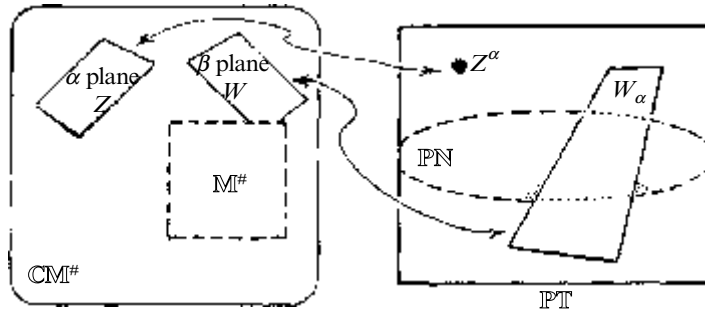
Fig. 33.13 Complex spacetime description of (generally non-null) twistors and dual twistors. For any non-zero twistor Z^\alpha , there always is a 2-complex-dimensional locus in \mathbb{CM}^\# of points incident with it, called an \alpha plane, which is everywhere self-dual. For any non-zero dual twistor W_\alpha , the points in \mathbb{CM}^\# incident with it always constitute 2-complex-dimensional plane which is anti-self-dual, called a \beta plane. Only for null twistors or null dual twistors are there any real points on these loci, and then the real points constitute a light ray, in accordance with Fig. 33.12.
