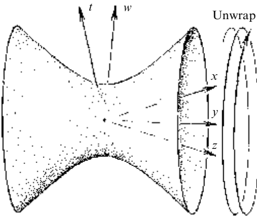
Fig. 28.8 Anti-de Sitter spacetime (pictured as a hyperboloid with two spatial dimensions suppressed) is a Lorentzian ‘4-sphere’ (of positive radius, giving an intrinsic metric signature + - - - ), in pseudo-Minkowskian 5-space (with metric ds^2 = dt^2 + dw^2 - dx^2 - dy^2 - dz^2 ). As defined, we have closed timelike curves, but these can be removed by infinitely ‘unwrapping’ in the (t, w) -plane.
