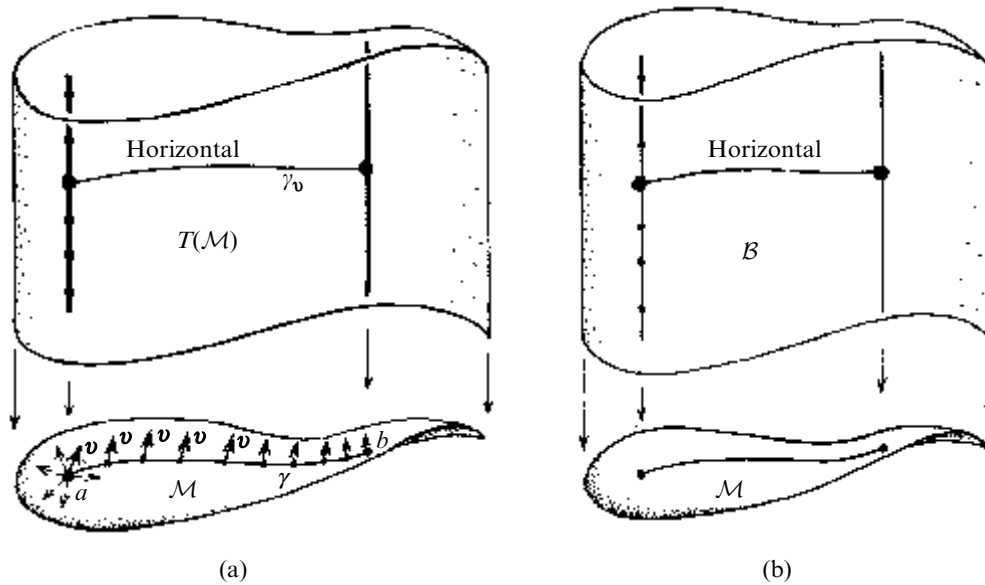
Fig. 15.17 Types of connection on a general manifold \mathcal{M} compared. (a) The original notion (§14.3), defining a notion of ‘parallel’ for tangent vectors transported along curves in \mathcal{M} , is described in terms of the tangent bundle T(\mathcal{M}) of \mathcal{M} (Fig. 15.12a). A particular tangent vector v at a point a of \mathcal{M} is represented in T(\mathcal{M}) by a particular point of the fibre above a . A ‘horizontal’ curve \gamma_v in T(\mathcal{M}) from this point represents the parallel transport of v along a curve \gamma in \mathcal{M} . (b) The same idea applies to a bundle \mathcal{B} over \mathcal{M} , other than T(\mathcal{M}) , where ‘constant transport’ in \mathcal{M} is defined from a notion of ‘horizontal’ in \mathcal{B} .
