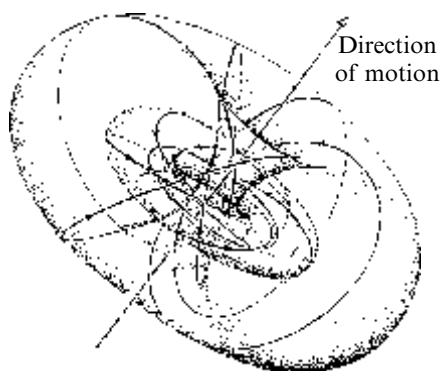
Fig. 33.15 A spatial picture giving a ‘snapshot’ of a Robinson congruence. (Stereographically projected Clifford parallels on S^3 , see Figs. 8.7a, 15.8, which is a 3-parameter family of circles—and one straight line—filling the whole of \mathbb{E}^3 .) We imagine a particle at each point of \mathbb{E}^3 , moving in a straight line with the speed of light (a light ray) in the direction of the (oriented) circle on which it lies. The whole configuration propagates with the speed of light in the (negative) direction of the straight line in the figure. This represents the motion and angular momentum of the spinning massless particle described by the Z^\alpha .
