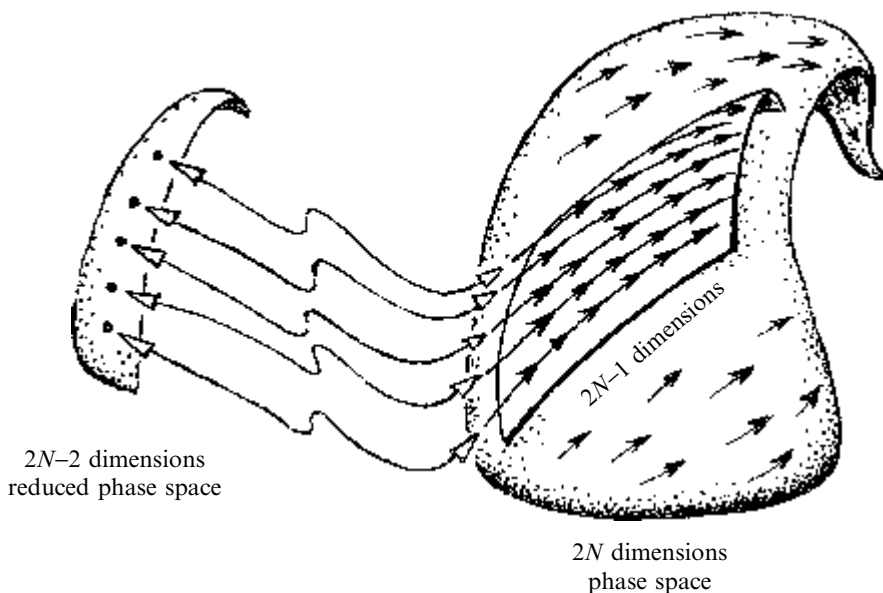
Fig. 20.8 Phase space T^*(\mathcal{C}) is a 2N -dimensional symplectic manifold, for an N -dimensional \mathcal{C} . For a given energy value (constant \mathcal{H} , as in Fig. 20.5), we have a (2N-1) -dimensional region containing a (2N-2) -dimensional family of the Hamiltonian flow trajectories. The reduced phase space, whose points represent these trajectories, is itself a 2(N-1) -dimensional symplectic manifold.
