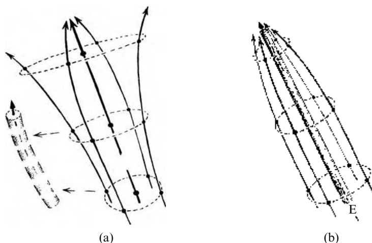
Fig. 17.9 Spacetime versions of Fig. 17.8 (in the Newton–Cartan picture \mathcal{N} of Fig. 17.7), in terms of the relative distortion of neighbouring geodesics. (a) Geodesic deviation in empty space (basically Weyl curvature of §19.7) as seen in the world lines of A and surrounding particles (one spatial dimension suppressed), as might be induced from the gravitational field of a nearby body E. (b) The corresponding inward acceleration (basically Ricci curvature) due to the mass density within the bundle of geodesics.
