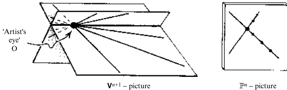
Fig. 15.15 To construct n -dimensional projective space \mathbb{P}^n , take an (n+1) -dimensional vector space \mathbf{V}^{n+1} , and regard \mathbb{P}^n as the space of the 1-dimensional vector subspaces of \mathbf{V}^{n+1} (lines through the origin of \mathbf{V}^{n+1} ). A straight line in \mathbb{P}^n is given by a 2-dimensional subspace of \mathbf{V}^{n+1} (plane through origin), collinear points of \mathbb{P}^n arising as lines through O in such a plane. This applies both to the real case ( \mathbb{RP}^n ) and the complex case ( \mathbb{CP}^n ). The geometry of \mathbb{RP}^2 formalizes the procedures of perspective in pictorial representation: consider the artist's eye to be at the origin O of \mathbf{V}^3 , taking \mathbf{V}^3 as the artist's ambient Euclidean 3-space. A light ray through O is viewed by the artist as single point. What the artist depicts as a 'straight line' ( \mathbb{RP}^1 in \mathbb{RP}^2 ) (on any particular choice of artist's canvas) indeed corresponds to the plane ( \mathbf{V}^2 ) joining that line to O . Pairs of planes through O always intersect, even when joining parallel lines in \mathbf{V}^3 to O . (For example, the two bottom boundary lines in the left-hand picture play the role of the road boundaries of Fig. 15.13.)
