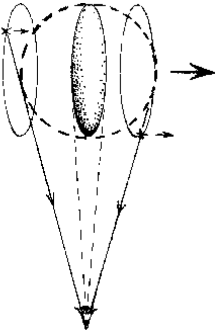
Fig. 18.15 The FitzGerald–Lorentz flattening is not directly visible because what appears to an observer to be the rear of the sphere involves a longer path length than what appears to be the front of the sphere (the rear part moving out of the way of the light and the front part moving into it). Accordingly, the apparent rear edge refers to an earlier position of the sphere than does the front edge, whereby the image is compensatingly stretched in the direction of motion.
