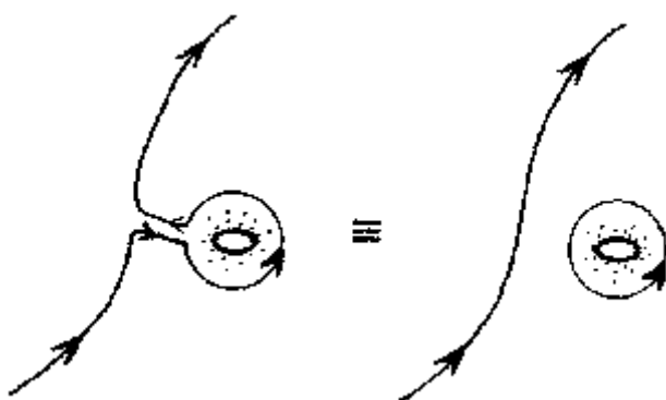
Fig. 7.2 With a homological deformation, parts of paths cancel each other, if traversed in opposite directions. Sometimes this gives rise to separated loops.
