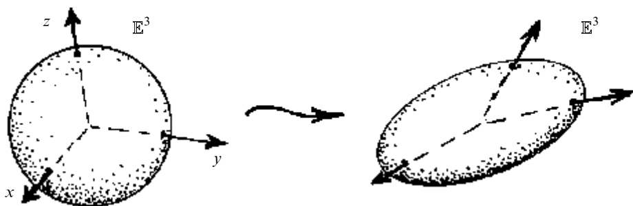
Fig. 13.5 A linear transformation acting on \mathbb{E}^3 (expressed in terms of Cartesian x, y, z coordinates) would generally squash or stretch the unit sphere x^2 + y^2 + z^2 = 1 into an ellipsoid. The orthogonal group O(3) consists of the linear transformations of \mathbb{E}^3 which preserve the unit sphere.
