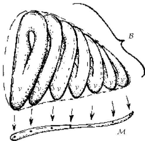
Fig. 15.2 A bundle \mathcal{B} , with base space \mathcal{M} and fibre \mathcal{V} may be thought of as constituted as an ‘ \mathcal{M} ’s worth of \mathcal{V} s’. The canonical projection from \mathcal{B} down to \mathcal{M} may be viewed as the collapsing of each fibre \mathcal{V} down to a single point.
