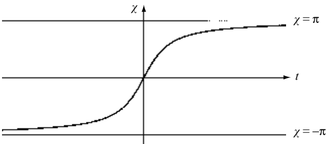
Fig. 9.8 Graph of t = \tan \chi/2 .
