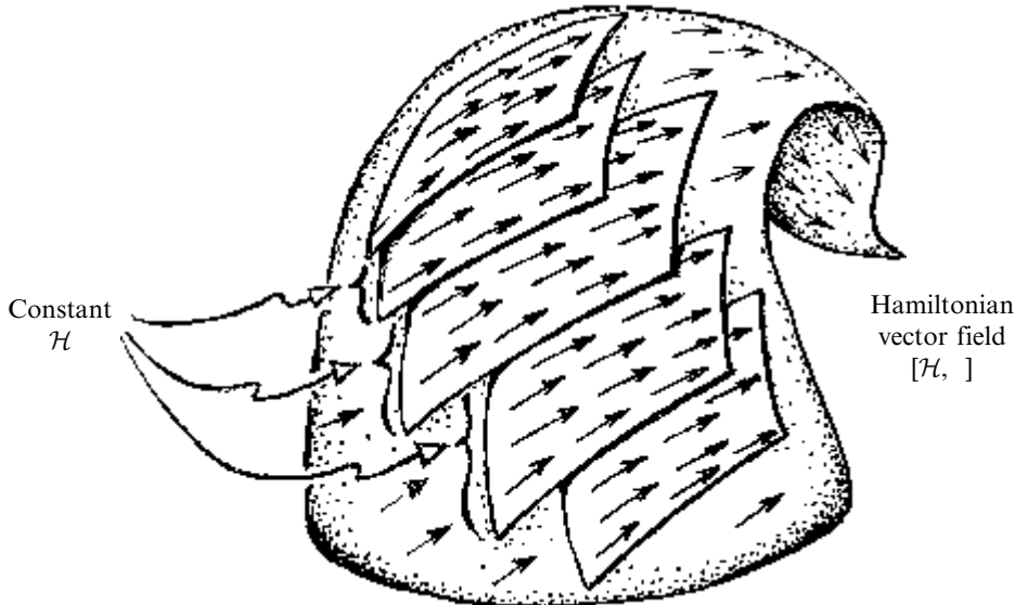
Fig. 20.5 The Hamiltonian flow \{\mathcal{H}, \cdot\} , representing the Newtonian time-evolution of the system (see §20.4), is a vector field on phase space T^*(C) . For the hypersurfaces of fixed \mathcal{H} -values (fixed energy, taking \mathcal{H} to be time independent), the trajectories remain within the fixed- \mathcal{H} hypersurface, in accordance with energy conservation.
