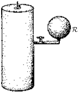
Fig. 27.3 A closed container, part of which is a bulb-shaped region \mathcal{R} whose volume is \frac{1}{10} of that of the entire container. How much does the entropy increase when a gas, initially all contained in \mathcal{R} , is allowed to flow into the entire volume?
