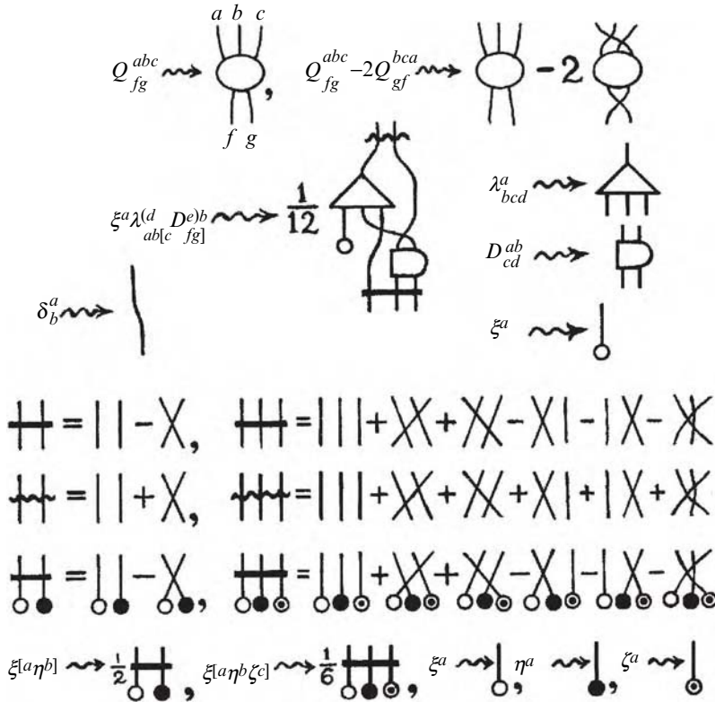
Fig. 12.17 Diagrammatic tensor notation. The \left[\begin{smallmatrix} 3 \\ 2 \end{smallmatrix}\right] -valent tensor Q is represented by an oval with 3 arms and 2 legs, where the general \left[\begin{smallmatrix} p \\ q \end{smallmatrix}\right] -valent tensor picture would have p arms and q legs. In an expression such as Q_{fg}^{abc} - 2Q_{gf}^{bca} , the diagrammatic notation uses positioning on the page of the ends of the arms and legs to keep track of which index is which, instead of employing individual index letters. Contractions of tensor indices are represented by the joining of an arm and a leg, as illustrated in the diagram for \xi^a \lambda_{ab[c}^{(d} D^{e)b}_{fg]} . This diagram also illustrates the use of a thick bar across index lines to denote antisymmetrization and a wiggly bar to represent symmetrization. The factor \frac{1}{12} in the diagram results from the fact that (to facilitate calculations) the normal factorial denominator for symmetrizers and antisymmetrizers is omitted in the diagrammatic notation (so here we need \frac{1}{2!} \times \frac{1}{3!} = \frac{1}{12} ). In the lower half of the diagram, antisymmetrizers and symmetrizers are written out as ‘disembodied’ expressions (by use of the diagrammatic representation of the Kronecker delta \delta_b^a that will be introduced in §13.3, Fig. 13.6c). This is then used to express the (multivector) wedge products \xi \wedge \eta and \xi \wedge \eta \wedge \zeta .
