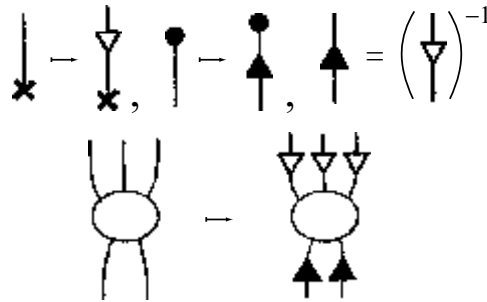
Fig. 13.13 The linear transformation x^a \mapsto T^a_b x^b , applied to \mathbf{x} in the vector space \mathbf{V} (with \mathbf{T} depicted as a white triangle), extends to the dual space \mathbf{V}^* by use of the inverse \mathbf{S} = \mathbf{T}^{-1} (depicted as a black triangle) and thence to the spaces \mathbf{V}^* \otimes \dots \otimes \mathbf{V}^* \otimes \mathbf{V} \otimes \dots \otimes \mathbf{V} of [^p_q] -valent tensors \mathbf{Q} . The case p = 3, q = 2 is illustrated, with \mathbf{Q} shown as an oval with three arms and two legs undergoing Q_{ab}{}^{cde} \propto S^{a'}_a S^{b'}_b T^c_{c'} T^d_{d'} T^e_{e'} Q_{a'b'}{}^{c'd'e'} .
