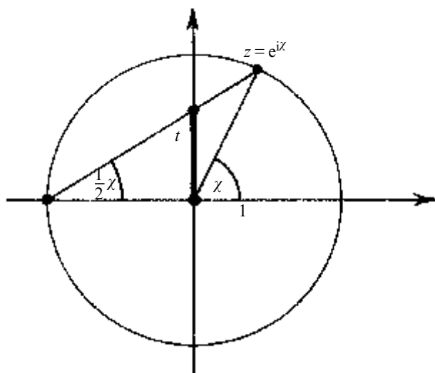
Fig. 9.9 Geometry of t = \tan \frac{\chi}{2} .
