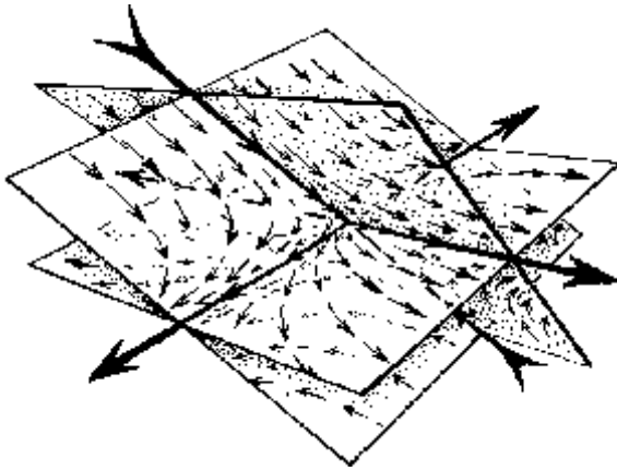
Fig. 13.10 The action of a linear transformation T . Its eigenvectors always constitute linear spaces through the origin (here three lines). These spaces are unaltered by T . (In this example, there are two (unequal) positive eigenvalues (outward pointing arrows) and one negative one (inward arrows).
