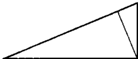
Fig. 2.9 Proof of the Pythagorean theorem using similar triangles. Take a right-angled triangle and drop a perpendicular from its right angle to its hypotenuse. The two triangles into which the original triangle is now divided have areas which sum to that of the original triangle. All three triangles are similar, so their areas are in proportion to the squares of their respective hypotenuses. The Pythagorean theorem follows.
