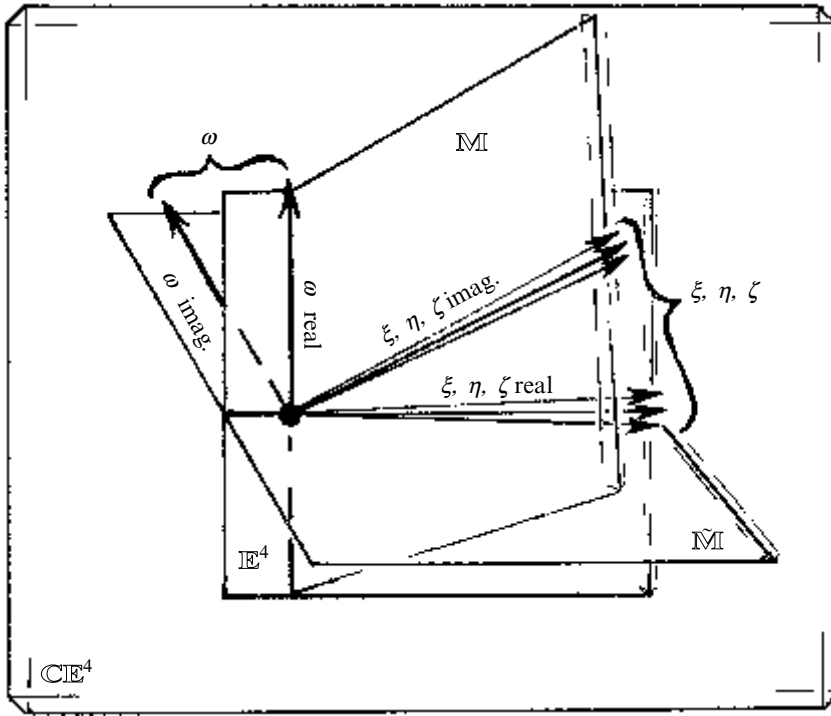
Fig. 18.2 Complex Euclidean space \mathbb{CE}^4 has a complex (holomorphic) metric ds^2 = d\omega^2 + d\xi^2 + d\eta^2 + d\zeta^2 in complex Cartesian coordinates (\omega, \xi, \eta, \zeta) . Euclidean 4-space \mathbb{E}^4 is the ‘real section’ for which \omega, \xi, \eta, \zeta are all real. Minkowski spacetime \mathbb{MI} , with the +- - - ds^2 metric, is a different real section, \omega being real and \xi, \eta, \zeta pure imaginary. We get another Lorentzian real section \tilde{\mathbb{MI}} by taking \omega to be pure imaginary and \xi, \eta, \zeta real, where the induced ds^2 now gives the +++- ‘ d\ell^2 ’ version of the Minkowski metric.
