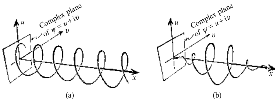
Fig. 21.5 A particle wavefunction: \psi as a complex function of position x . (a) Momentum state e^{-iP_x/\hbar} , depicted as a corkscrew (eigenfunction of momentum p ). (b) A wave packet e^{-A^2 x^2} e^{-iP_x/\hbar} .
