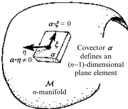
Fig. 12.7 A (non-zero) covector \alpha at a point of \mathcal{M} , determines an (n-1) -dimensional plane element there. The vectors \xi satisfying \alpha \cdot \xi = 0 define the directions within it.
