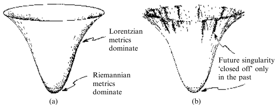
Fig. 28.18 The Hartle–Hawking ‘no-boundary’ proposal suggests that (a) the Big Bang can be treated according to a quantum-gravity procedure whereby Riemannian (rather than Lorentzian) geometries dominate the path integral near the classical singularity, and provide ways of closing off the spacetime in a non-singular way. (b) With regard to the singularities of collapse, the ‘closing off’ seems to be required only at the ‘far end’ of the spacetime, thereby allowing the high-entropy generic singularities that are expected to occur in gravitational collapse to black holes (i.e. Big Crunch).
