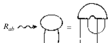
Fig. 19.7 Diagrammatic notation for Ricci-tensor definition R_{ab} = R_{acb}{}^c (see Fig. 14.21).
