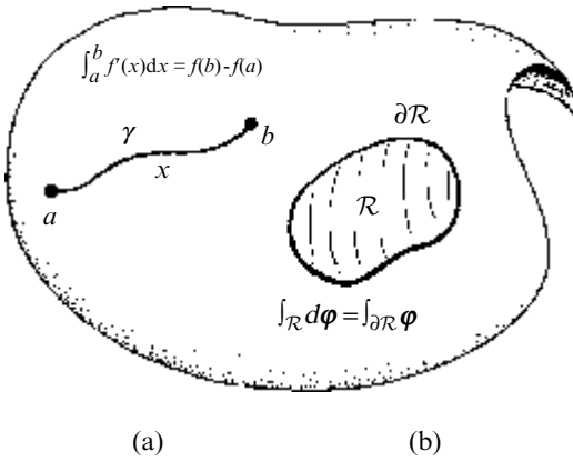
Fig. 12.11 The fundamental theorem of exterior calculus \int_{\mathcal{R}} d\varphi = \int_{\partial\mathcal{R}} \varphi . (a) The classical (17th century) case \int_a^b f'(x)dx = f(b) - f(a) , where \varphi = f(x) and \mathcal{R} is the segment of a curve \gamma from a to b , parametrized by x , so \partial\gamma consists of \gamma 's end-points x = a (counting negatively) and x = b (positively). (b) The general case, for a p -form \varphi , where \mathcal{R} is a compact oriented (p+1) -dimensional region with p -dimensional boundary \partial\mathcal{R} .
