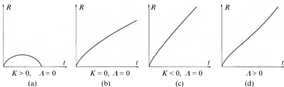
Fig. 27.15 Graphs of R = R(t) for Friedmann models, first with \Lambda = 0 : (a) K > 0 , (b) K = 0 , (c) K < 0 , and then (d) with \Lambda > 0 . (Case (d) is plotted for K = 0 , but the other cases are very similar, provided that \Lambda is large enough in relation to spatial curvature.)
