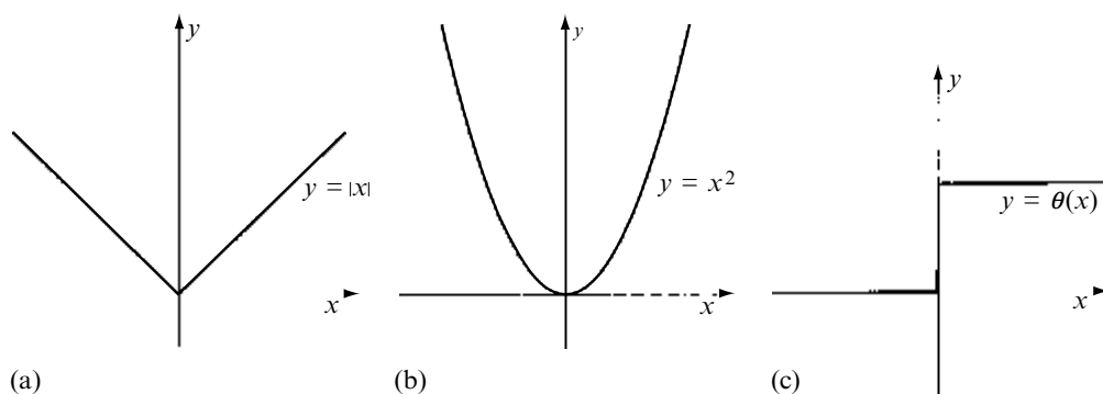
Fig. 6.2 Graphs of (a) |x| , (b) x^2 , and (c) \theta(x) ; the domain and target being the system of real numbers in each case.
