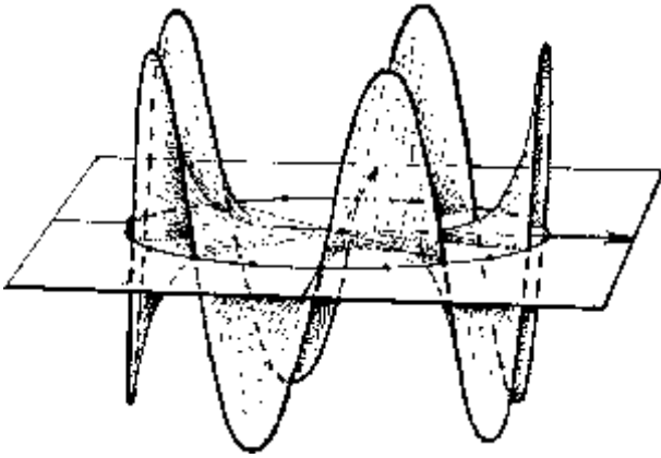
Fig. 9.4 On the unit circle, the real and imaginary parts of the function z^n appear as n th harmonic cos and sin waves (the real and imaginary parts of e^{inx} , respectively, where z = e^{ix} ). Here, for n = 5 , the real part of z^5 is plotted.
