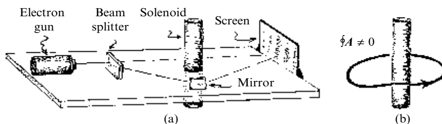
Fig. 19.6 Aharonov–Bohm effect. (a) A beam of electrons is split into two paths that go to either side of a collection of lines of magnetic flux (achieved by means of a long solenoid). The beams are brought together at a screen, and the resulting quantum interference pattern (compare Fig. 21.4) depends upon the magnetic flux strength—despite the fact that the electrons only encounter a zero field strength ( \mathbf{F} = 0 ). (b) The effect depends on the value of \oint A , which can be non-zero over the relevant topologically non-trivial closed path despite \mathbf{F} vanishing over this path. The quantity \oint A is unchanged for continuous deformations of the path within the field-free region.
