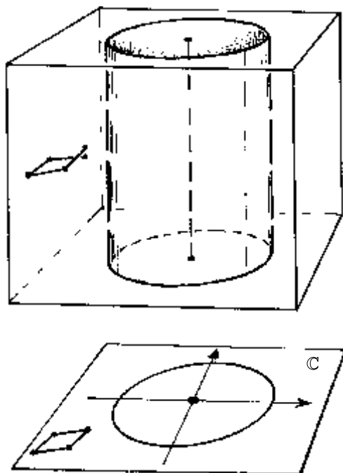
Fig. 15.19 To obtain a local path dependence (with curvature), in our bundle (now B^{\mathbb{C}} ), we need at least 2 dimensions in the base \mathcal{M}^{\mathbb{C}} , now taken as the complex plane \mathbb{C} , where the S^1 of Fig. 15.16 is its unit circle. The fibres are to remain \mathbf{V}^1 (i.e. modelled on the real line \mathbb{R} ). Using z as a complex coordinate for \mathbb{C} = \mathcal{M}^{\mathbb{C}} , we use the explicit connection \nabla = \partial/\partial z - A , where A is a complex smooth function of z . When A is holomorphic the bundle curvature vanishes, but if A = ikz (with suitable k ), we get the strained bundle of Fig. 15.16 for the part over the unit circle. The bundle curvature is manifested in the failure to close of a horizontal polygon above a small parallelogram in \mathcal{M}^{\mathbb{C}} .
