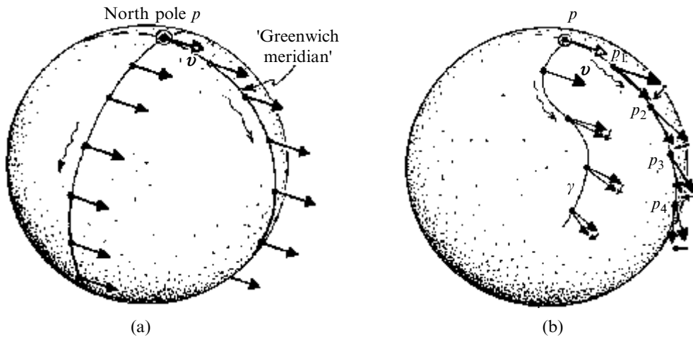
Fig. 14.2 Parallelism on the sphere S^2 . Choose p at the north pole, with tangent vector \mathbf{v} pointing along the Greenwich meridian. Which tangent vectors, at other points of S^2 , are we to regard to being ‘parallel’ to \mathbf{v} ? (a) The direct Euclidean notion of ‘parallel’, from the embedding of S^2 in \mathbb{E}^3 , does not work because (except along the meridian perpendicular to the Greenwich meridian) the parallel \mathbf{v} s do not remain tangent to S^2 . (b) Remedy this, moving \mathbf{v} parallel along a given curve \gamma , by continually projecting back to tangency with the sphere. (Think of \gamma as made up of large number of tiny segments p_0 p_1, p_1 p_2, p_2 p_3, \dots , projecting back at each stage. Then take the limit as the segments are made smaller and smaller.) This notion of parallel transport is indicated for the Greenwich meridian, but also for a general curve \gamma .
