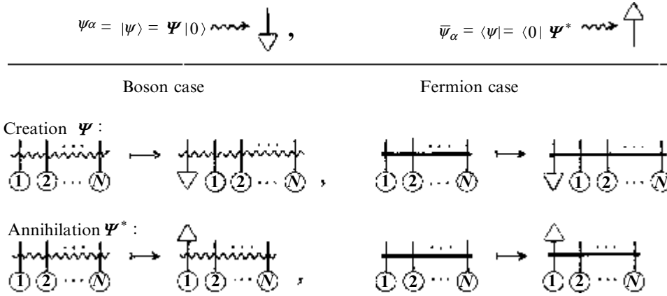
Fig. 26.1 Diagrammatic form of the action of a creation operator \Psi in the boson case \phi_1^{(\beta)}\phi_2^{(\gamma)}\dots\phi_N^{(\nu)}\mapsto\psi^{(\alpha)}\phi_1^{(\beta)}\phi_2^{(\gamma)}\dots\phi_N^{(\nu)} and in the fermion case \phi_1^{[\beta]}\phi_2^{(\gamma)}\dots\phi_N^{[\nu]}\mapsto\psi^{[\alpha]}\phi_1^{(\beta)}\phi_2^{(\gamma)}\dots\phi_N^{[\nu]} ; and of an annihilation operator \Psi^* in the boson case \phi_1^{(\alpha)}\phi_2^{(\beta)}\dots\phi_N^{(\mu)}\mapsto\bar{\psi}_\alpha\phi_1^{(\alpha)}\phi_2^{(\beta)}\dots\phi_N^{(\mu)} and in the fermion case \phi_1^{[\alpha]}\phi_2^{(\beta)}\dots\phi_N^{[\mu]}\mapsto\bar{\psi}_\alpha\phi_1^{[\alpha]}\phi_2^{(\beta)}\dots\phi_N^{[\mu]} .
