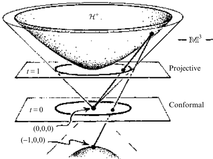
Fig. 18.10 In Minkowski 3-space \mathbb{M}^3 , the hyperbolic 2-geometry of \mathcal{H}^+ (given by t^2 - x^2 - y^2 = 1 ) directly relates to Beltrami's conformal and projective representations (illustrated in Figs. 2.11 and 2.16 respectively—M.C.Escher's print and in its distorted version). Beltrami's projective ('Klein') model is obtained by projecting \mathcal{H}^+ from the origin (0,0,0) to the interior of the unit circle in the plane t = 1 . Beltrami's conformal (Poincaré) model is obtained by projecting \mathcal{H}^+ from (-1,0,0) to the interior of the unit circle in t = 0 . (See also Beltrami's geometry of Fig. 2.17.) The analogous construction works also for hyperbolic 3-geometry in \mathbb{M} .
