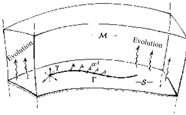
Fig. 32.1 Ashtekar’s original canonical variables, defined on a spacelike 3-surface S in spacetime \mathcal{M} , takes the ‘position’ parameters \Gamma to be the components of the 4-space spin-connection, restricted to S (for spinors \alpha^A , indicated by half-arrows). The ‘momentum’ parameters are basically the components of the (inverse) intrinsic metric \gamma of S (expressed as 2-forms and referred to an orthonormal basis at each point of S ).
