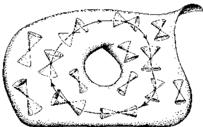
Fig. 17.18 The causality structure of \mathcal{E} is determined by g (as with \mathbb{M} , see Fig. 17.16), so extreme unphysical situations with ‘closed timelike curves’ might hypothetically arise, allowing future-directed signals to return from the past.
