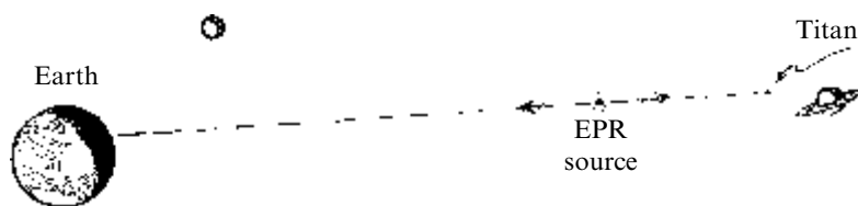
Fig. 23.4 The author, situated on the Earth, imagines himself to be the receiver of one component of a succession of EPR particle pairs, the other being a colleague on Titan, where the source of the pairs is roughly equidistant between the two receivers. Even for particles travelling at the speed of light, there would be about 45 minutes to decide on the detector orientations.
