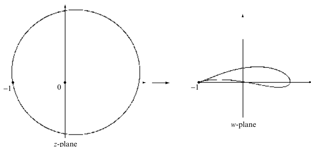
Fig. 8.15 Zhoukowsky's transformation w = \frac{1}{2}(z + 1/z) takes the exterior of a circle through z = -1 to an aerofoil cross-section, enabling the airflow pattern about the latter to be calculated.
