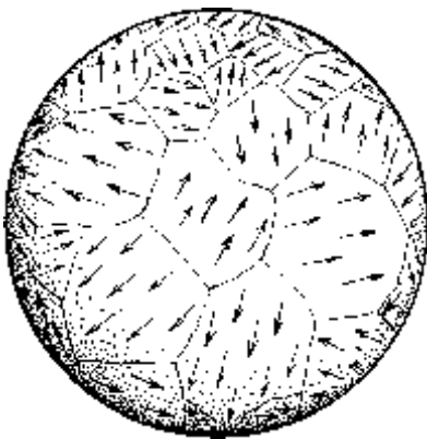
Fig. 28.2 Ideally, when a ferromagnet slowly cools from its Curie point, the directions of magnetization of its atom would all settle in the same (arbitrary) direction. But in practice (or with too rapid cooling), we get a ‘patchwork’ of such directions of magnetization.
