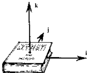
Fig. 11.2 We can think of the quaternionic operators \mathbf{i} , \mathbf{j} , and \mathbf{k} as referring to rotations (through 180^\circ , i.e. \pi ) of some object, which is here taken to be a book.
