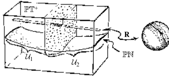
Fig. 33.16 The basic twistor contour integral. A twistor function f (for helicity \frac{1}{2}n ), homogeneous of degree -n-2 , is multiplied n times by \pi ( n positive) or acted upon -n times by \partial/\partial\omega ( n negative), these supplying the indices, and then multiplied by the 2-form \tau = d\pi_0 \wedge d\pi_1 . For any particular choice of spacetime point R , with position vector r , a contour integral is then performed in the region \mathbf{R} of twistor space defined by the incidence relation \omega = i\mathbf{r}\pi . This integrates out the \pi -dependence, and we are left with a solution of the massless field equations. In the case illustrated, \mathbf{R} is taken in the top half of twistor space \mathbb{PT}^+ (or \mathbb{T}^+ ) and f is holomorphic in the intersection of \mathcal{U}_1 and \mathcal{U}_2 , where the open sets \mathcal{U}_1 and \mathcal{U}_2 , together cover the whole of \mathbb{PT}^+ (or \mathbb{T}^+ ).
