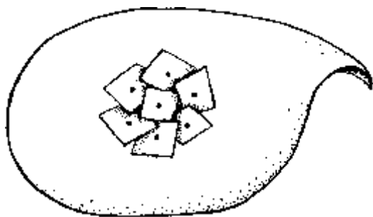
Fig. 12.8 The (n - 1) -plane elements defined by a covector field \alpha would, in general, twist around in a way that prevents them from consistently touching a single family of (n - 1) -surfaces—although in the particular case \alpha = d\Phi (for a scalar field \Phi ), they would touch the surfaces \Phi = \text{const.} (generalizing the ‘contour lines’ of Fig. 10.8).
