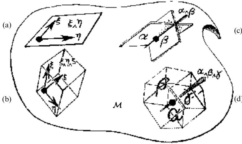
Fig. 12.10 (a) A 2-plane element at a point of \mathcal{M} , being spanned by independent vectors \xi, \eta , is described by the bivector \xi \wedge \eta . (b) Similarly, a 3-plane element spanned by \xi, \eta, \zeta is described by \xi \wedge \eta \wedge \zeta . (c) Dually, an (n-2) -plane element, the intersection of two (n-1) -plane elements specified by 1-forms \alpha, \beta , is described by \alpha \wedge \beta . (d) The (n-3) -plane element of intersection of the three (n-1) -plane elements specified by \alpha, \beta, \gamma , is described by \alpha \wedge \beta \wedge \gamma .
