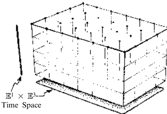
Fig. 17.2 Aristotelian spacetime \mathcal{A} = \mathbb{E}^1 \times \mathbb{E}^3 is the space of pairs (t, \mathbf{x}) , where t (‘time’) ranges over a Euclidean 1-space \mathbb{E}^1 , and \mathbf{x} (‘point in space’) ranges over a Euclidean 3-space \mathbb{E}^3 .
