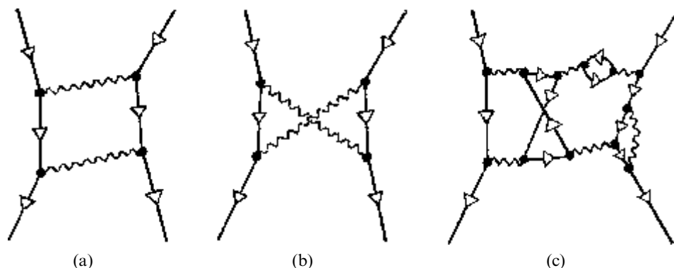
Fig. 26.7 Higher-order processes giving corrections to Møller scattering. (a) and (b) depict 2-photon exchanges between two electrons, while (c) is a much higher-order process involving internal pair creations and annihilations. Each such Feynman graph represents an integral, and the contributions from all of them must be added up.
