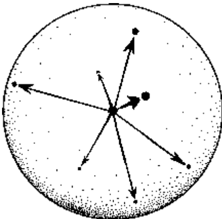
Fig. 22.14 Majorana’s description of the general (projective) spin state for a massive particle of spin \frac{n}{2} , given by n unordered points on the Riemann sphere. We can think of the vectors out from the centre to each of these points to be contributing spin \frac{1}{2} , in accordance with the prescription of Fig. 22.10. The symmetrical product of these spins gives the total. (In 2-spinor notation, the complete spin state is the symmetric n -valent spinor, which factorizes \psi_{AB\dots F} = \alpha_{(A}\beta_{B}\cdots\varphi_{F)} , where \alpha_A, \beta_A, \dots, \varphi_A , determine the n points, as in Fig. 22.10.)
