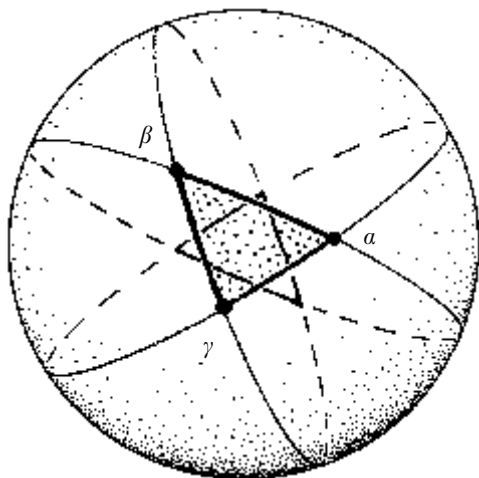
Fig. 2.20 Hariot’s formula for the area of a spherical triangle , with angles \alpha, \beta, \gamma , is \Delta = R^2(\alpha + \beta + \gamma - \pi) . Lambert’s formula, for a hyperbolic triangle, has C = -1/R^2 .
