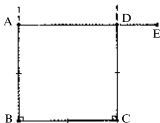
Fig. 2.7 Try to construct a square. Take ABC and BCD as right angles, with AB = BC = CD . Does it follow that DA is also equal to these lengths and that DAB and CDA are also right angles?
