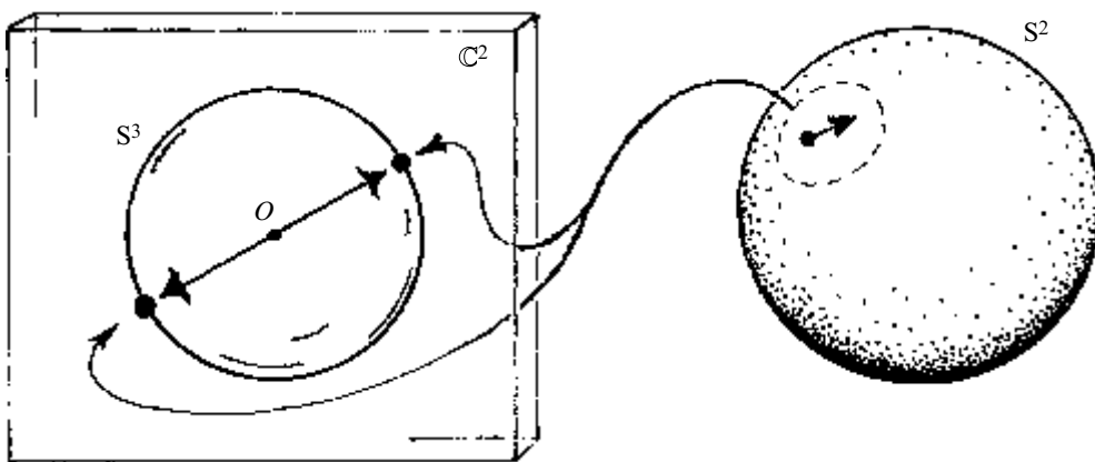
Fig. 15.10 The bundle \mathcal{B}' of unit tangent vectors to S^2 is a slight modification of the Clifford bundle, where antipodal points of S^3 are identified. Without this identification, we obtain S^3 as the (Clifford) bundle \mathcal{B} of spinorial tangent vectors to S^2 . The fibres of \mathcal{B}' are still circles, but each circle-fibre of \mathcal{B} wraps twice around each circle-fibre of \mathcal{B}' .
