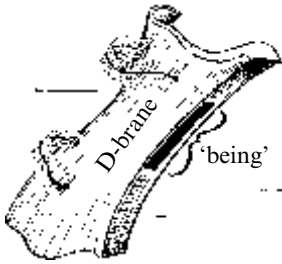
Fig. 31.17 An alternative viewpoint to that of Fig. 31.3, often expressed in the context of D-branes, is that a ‘being’ in higher dimensional space need not straddle all the extra dimensions but may be thought of as ‘living’ in a subspace, perhaps on a D-brane boundary
