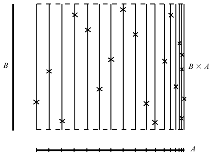
Fig. 16.5 For general sets A , B , the set of all mappings from A to B is denoted B^A (see also Fig. 6.1). Each element of A is assigned a particular element of B . This provides a cross-section of B \times A , regarded as a bundle over A (as in Fig. 15.6a), except that there is no notion of continuity involved.
