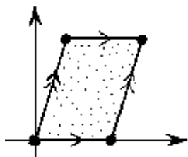
Fig. 8.10 To construct a Riemann surface of genus 1, take a region of the complex plane bounded by a parallelogram, vertices 0, 1, 1+p , p (cyclicly), with opposite edges identified. The quantity p provides a modulus for the Riemann surface.
