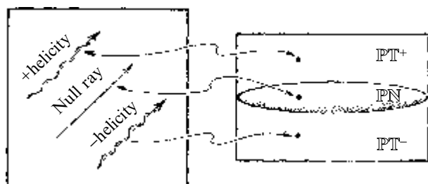
Fig. 33.6 The real 5-manifold \mathbb{IPN} divides projective twistor space \mathbb{IPT} into two complex-3-manifold pieces \mathbb{IPT}^+ and \mathbb{IPT}^- , these representing massless particles of positive and of negative helicity, respectively.
