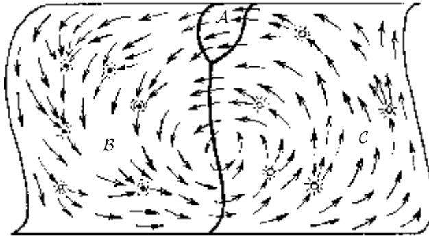
Fig. 30.19 Phase-space description of Hawking's box, with arrows describing (Hamiltonian) evolution (of the processes involved in Fig. 30.18). The regions \mathcal{A}, \mathcal{B}, \mathcal{C} , correspond, respectively, to (a), (b), (c) in Fig. 30.18. Accordingly, a black hole is present for region \mathcal{B} , but not for region \mathcal{C} . The presence of a black hole results in a confluence of flow lines (reduction of phase-space volume), according to LOSS, owing to information destruction at the black hole's (future) singularity. There is a compensating creation of flow lines (increase in phase-space volume) involved in the time-asymmetry of the R process (assumed to be objectively real); see Fig. 30.1. The proposal is that there should be an overall balance between these two Liouville-theorem violating processes, giving ultimate phase-space volume preservation in the flow.
