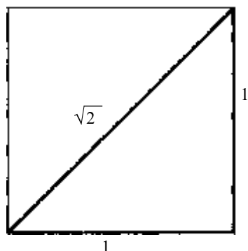
Fig. 3.1 A square of unit side-length has diagonal \sqrt{2} , by the Pythagorean theorem.
