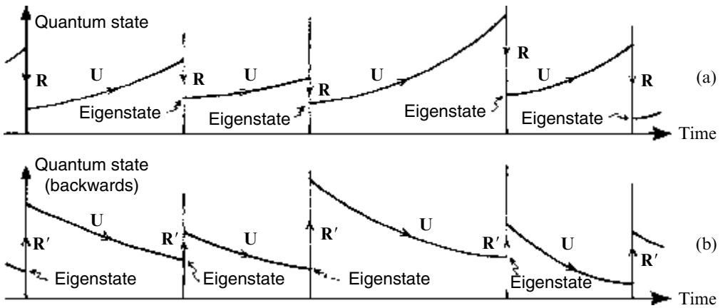
Fig. 30.2 Schematic illustration of the alternation... U , R , U , R , U ,... of the two processes U and R as used in practice in quantum mechanics (compare Fig. 22.1), according to: (a) standard time-direction of evolution, where operator eigenstates occur at the past end of each stretch of U -evolution, and (b) time-reversed viewpoint of evolution, where operator eigenstates occur at the future end of each stretch of U -evolution. In the 'transactional' interpretation of quantum mechanics, there are two state vectors, one evolving according to (a) and the other according to (b).
