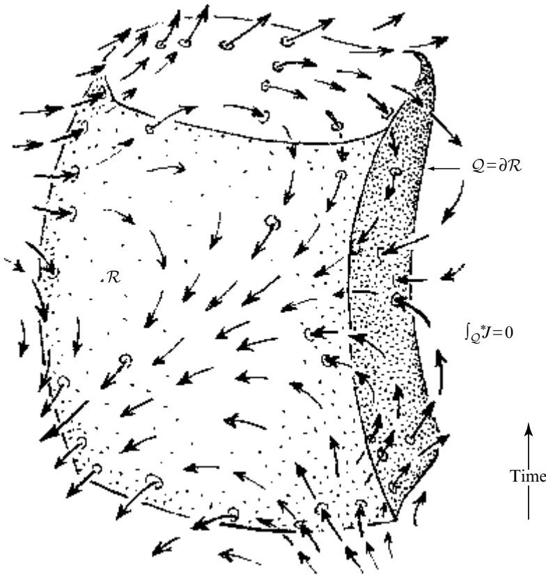
Fig. 19.3 Conservation of electric charge in spacetime. The closed 3-surface Q is the boundary Q = \partial \mathcal{R} of a compact 4-volume \mathcal{R} , in Minkowski spacetime \mathbb{M} , so the fundamental theorem of exterior calculus tells us \int_Q \mathbf{J} = \int_{\mathcal{R}} d^* \mathbf{J} = 0 , since d^* \mathbf{J} = 0 . The quantity \mathbf{J} describes the ‘flux’ (or ‘flow’) of charge across Q , so the total charge flowing in across Q is equal to that flowing out, expressing charge conservation.
