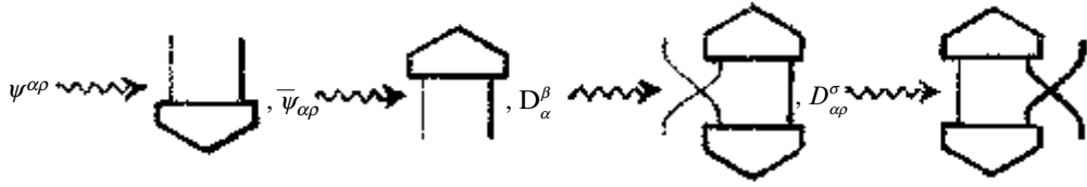
Fig. 29.5 Diagrammatic notation for density matrices constructed by ‘summing over unknown states’. The normalized ket-vector |\psi\rangle is expressed as \psi^{\alpha\rho} , where ‘ \alpha ’ refers to ‘here’ (Earth) and ‘ \sigma ’ refers to ‘there’ (Titan). The Hermitian conjugate (bra-vector \langle\psi| ) is \bar{\psi}_{\alpha\rho} and the normalization is \bar{\psi}_{\alpha\rho}\psi^{\alpha\rho} = 1 . The density matrix used ‘here’ is D_{\alpha}^{\beta} = \psi_{\alpha\rho}\psi^{\beta\rho} , while that used ‘there’ is \tilde{D}_{\rho}^{\sigma} = \bar{\psi}_{\alpha\rho}\psi^{\alpha\sigma} .
