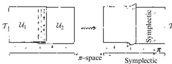
Fig. 33.25 Apply the idea of Fig. 33.24 in case of the twistor description of anti-self-dual gravity (with two patches). The vector field is (\partial f / \partial \omega^0) \partial / \omega^1 - (\partial f / \partial \omega^1) \partial / \omega^0 , with f homogeneous of degree 2. We get a curved twistor space (portion) \mathcal{T} . There is a global projection of \mathcal{T} to the \pi -space. Each fibre of this projection is a complex symplectic 2-space, as is the \pi -space itself.
