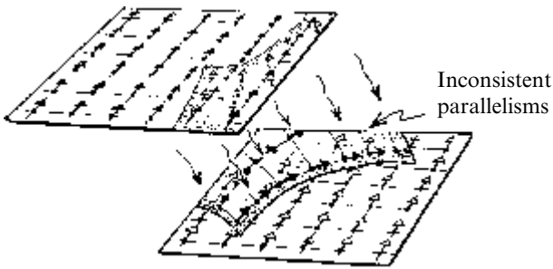
Fig. 14.1 The Euclidean notion of ‘parallel’ is likely to be inconsistent on the overlap between coordinate patches.
