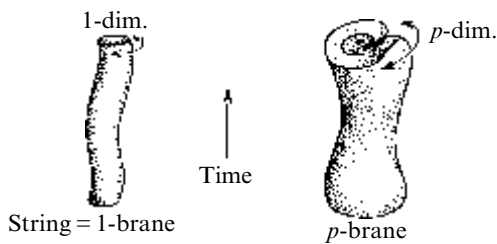
Fig. 31.13 Membranes (or p -branes, or just branes), have p spatial dimensions and 1 time dimension, the world-sheet being (1 + p) -dimensional. These structures are involved, together with ordinary strings (1-branes), as part of the undefined M-theory.
