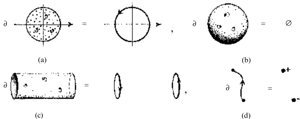
Fig. 12.16 The boundary \partial\mathcal{R} of a well-behaved compact oriented (p+1) -dimensional region \mathcal{R} is a (compact oriented) p -dimensional region (possibly empty), consisting of those points of \mathcal{R} that do not lie in the (p+1) -dimensional interior. (a) The boundary of the closed unit disc (given by |z| \leq 1 in the complex plane \mathbb{C} ) is the unit circle. (b) The boundary of the unit sphere is empty ( \emptyset denoting the empty set, see §3.4). (c) The boundary of a finite length of cylindrical surface consists of the two circles at either end, the orientation of each being opposite. (d) The boundary of a finite curve segment consists of two end-points, one positive and the other negative.
