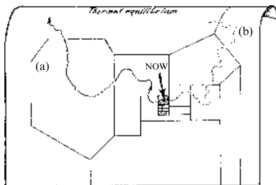
Fig. 27.6 The Second Law in action. The evolution of a physical system is represented by some curve in phase space. (a) If we know that at the moment NOW, our system is represented by a point x in a box \mathcal{V} of very small volume V , and we try to see what would be its probable future behaviour, we conclude, because of the vast discrepancies in box volumes, that, in the absence of any great bias in its motion, it will almost certainly enter larger and larger boxes, in accordance with the Second Law. (b) But suppose we apply this argument into the past , asking for the most probable way that the curve found its way into \mathcal{V} in the first place. The same argument seems to lead to the apparently absurd conclusion that the most likely way was that x simply found its way into \mathcal{V} from boxes that become progressively larger as we proceed into the past, in blatant contradiction with the Second Law.
