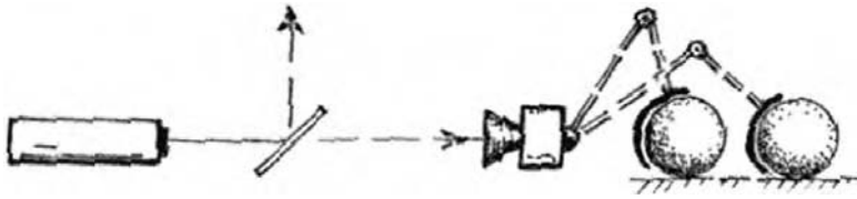
Fig. 30.20 Schrödinger's 'cat' of Fig. 29.7, but now the resulting quantum superposition is merely between two slightly differing locations of a lump of matter.
