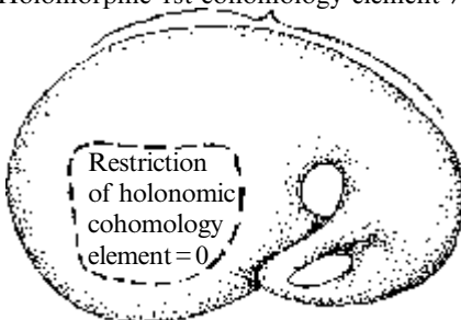
Fig. 33.20 A cohomology element can always be restricted down to a smaller region. But if this region is sufficiently small, the cohomology always disappears. This illustrates the non-locality of cohomology.
