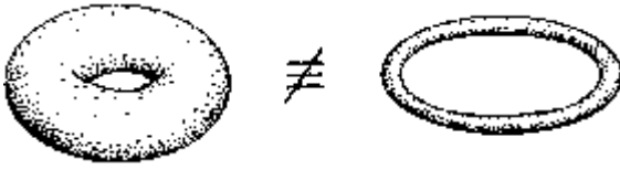
Fig. 8.11 Two inequivalent torus-topology Riemann surfaces.
