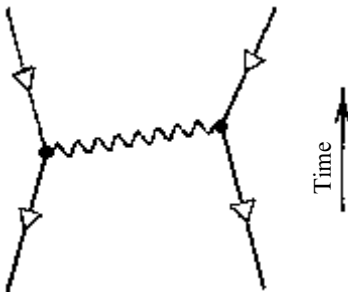
Fig. 26.5 Møller scattering of electrons: the most primitive quantum manifestation of the electrostatic (Coulomb) force between two charged particles. The electrostatic force comes about, here, from the ‘exchange’ of a single photon (wiggly line) between two electrons. The photon is necessarily ‘off shell’ and therefore virtual, as follows from 4-momentum conservation at each vertex.
