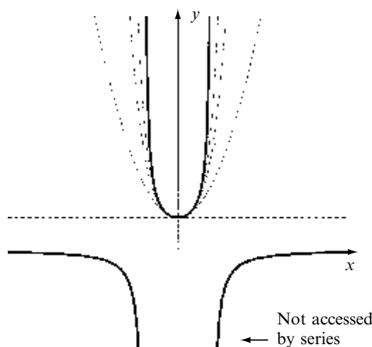
Fig. 4.1 The respective partial sums, 1 , 1 + x^2 , 1 + x^2 + x^4 , 1 + x^2 + x^4 + x^6 of the series for (1 - x^2)^{-1} are plotted, illustrating the convergence of the series to (1 - x^2)^{-1} for |x| < 1 and divergence for |x| > 1 .
