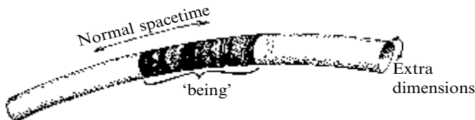
Fig. 31.3 Hosepipe model of a Kaluza–Klein-type higher-dimensional spacetime (see Fig. 15.1), where the dimension along the length of the hosepipe represents normal 4-spacetime and the dimension around the pipe represents the ‘small’ (perhaps Planck-scale) extra dimensions. We imagine a ‘being’ who inhabits this world, as straddling these ‘small’ extra dimensions, and so is not actually aware of them.
