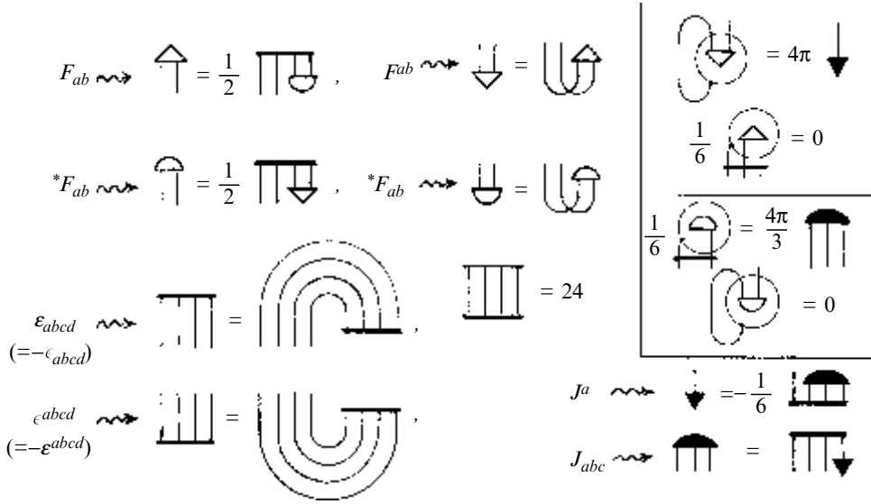
Fig. 19.1 Diagrams for Hodge duals and Maxwell equations. The quantities \epsilon_{abcd} (= \epsilon_{[abcd]}) and \epsilon^{abcd} (= \epsilon^{[abcd]}) , normalized so that \epsilon_{0123} = \epsilon^{0123} = 1 in a standard Minkowski frame, are related to their raised/lowered versions (via g^{ab} and g_{ab} ) by \epsilon_{abcd} = -\epsilon_{abcd} and \epsilon^{abcd} = -\epsilon^{abcd} . In the diagrams (left middle, lower two lines) this sign change is absorbed by an effective index reversal. Boxed off at the top right are the Maxwell equations, first using the field tensor F (with its raised form F^{ab} = g^{ac}g^{bd}F_{cd} ; cf. Fig. 14.21) so the equations are \nabla_a F^{ab} = 4\pi J^b , \nabla_{[a} F_{bc]} = 0 , and beneath that, correspondingly using the dual *F (where *F_{ab} = \frac{1}{2}\epsilon_{abcd}F^{cd} , *J_{abc} = \epsilon_{abcd}J^d ) so the equations are \nabla_{[a} F_{bc]} = \frac{4\pi}{3} *J_{abc} , \nabla_a *F^{ab} = 0 .
