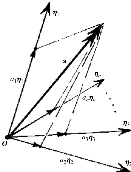
Fig. 11.5 Each basis element \boldsymbol{\eta}_1, \boldsymbol{\eta}_2, \boldsymbol{\eta}_3, \dots, \boldsymbol{\eta}_n , of a Grassmann algebra defines a vector in n -dimensional space, at some origin-point O . These vectors can be along the different coordinate axes (which can be ‘oblique’ axes; Grassmann algebra not being concerned with orthogonality). A general vector at O is a linear combination \mathbf{a} = a_1 \boldsymbol{\eta}_1 + a_2 \boldsymbol{\eta}_2 + \cdots + a_n \boldsymbol{\eta}_n .
