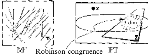
Fig. 33.14 We can obtain a ‘real’ picture of a non-null twistor Z^\alpha by first passing to its complex conjugate \bar{Z}_\alpha , thus defining a complex projective plane in \mathbb{P}^3\mathbb{T} . This plane is fixed by its intersection with \mathbb{P}\mathbb{N} , which is a 3-real-dimensional locus. This locus defines a 3-parameter family of light rays in \mathbb{M}^\# called a Robinson congruence.
