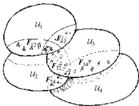
Fig. 33.17 Recall (from Fig. 12.5a) how a manifold is constructed from several coordinate patches. (Defined on each overlap between a pair of patches is a ‘transition function’, providing the ‘gluing’ of the patches.) Here, we consider transition functions which differ only infinitesimally from the identity, and therefore given by a vector field F_{ij} on each overlap of patches U_i, U_j , telling us how each patch is to ‘shunt’ relative to the others which it overlaps. (The ‘patches’ are open sets U_1, U_2, U_3, \dots on the flat coordinate space.)
