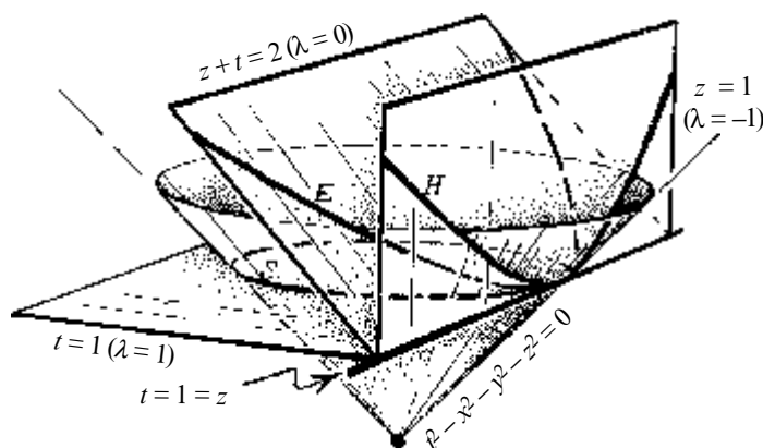
Fig. 18.9 Sections of the light cone t^2 - x^2 - y^2 - z^2 = 0 , by 3-planes (z + t) + \lambda(t - z) = 2 , through the 2-plane t = 1 = z . The coordinate y is suppressed, so dimensions appear reduced by 1. When \lambda > 0 the section S has a 2-sphere d\ell^2 metric, illustrated by the horizontal case \lambda = 1 . When \lambda = 0 we get the flat Euclidean d\ell^2 metric of the paraboloidal section E . When \lambda < 0 we get a hyperbolic d\ell^2 metric, illustrated by the vertical hyperbolic section H , in the case \lambda = -1 .
