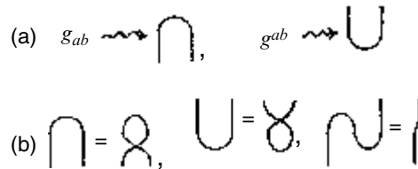
Fig. 13.15 (a) The metric g_{ab} and its inverse g^{ab} in the ‘hoop’ diagrammatic notation. (b) The relations g_{ab} = g_{ba} (i.e. \mathbf{g}^T = \mathbf{g} ), g_{ab} = g^{ba} , and g_{ab} g^{bc} = \delta_a^c in diagrammatic notation.
