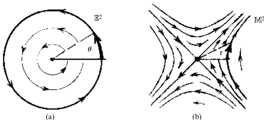
Fig. 30.5 Periodicity in imaginary time, illustrated by Minkowski 2-space \mathbb{M}^2 , complexified to \mathbb{CM}^2 = \mathbb{C}\mathbb{E}^2 . (a) The Euclidean plane \mathbb{E}^2 is one real section of the complex space \mathbb{CM}^2 . The Killing vector \partial/\partial\theta generates rotations in \mathbb{E}^2 , where we take polar coordinates (r, \theta) . Any function that is single-valued on \mathbb{E}^2 must be periodic in \theta with period 2\pi . (b) In the Lorentzian real section \mathbb{M}^2 of \mathbb{CM}^2 , the ‘Rindler’ (uniform-acceleration) time coordinate is \tau = i\theta (an analogue of the Schwarzschild time that is natural for a black hole), and a function that is analytic at the origin O must have an imaginary period in \tau , with period 2\pi i . (Killing vector \kappa = \partial/\partial\tau = -i\partial/\partial\theta .)
