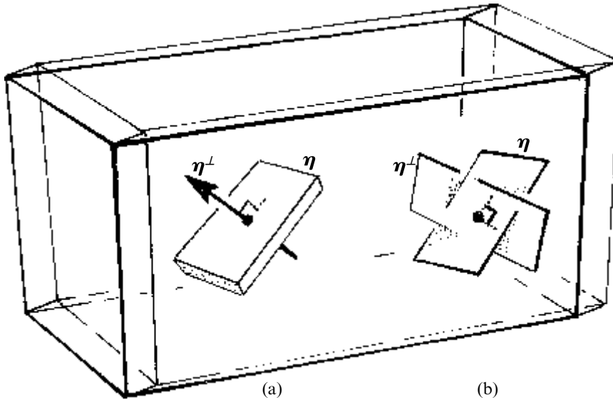
Fig. 18.4 In \mathbb{E}^4 , an r -plane element \boldsymbol{\eta} at a point p has an orthogonal complement \boldsymbol{\eta}^\perp which is a (4 - r) -plane element, where \boldsymbol{\eta} and \boldsymbol{\eta}^\perp never have a direction in common. (a) In particular, if \boldsymbol{\eta} is a 3-plane element, then \boldsymbol{\eta}^\perp is the normal direction to it. (b) If \boldsymbol{\eta} is a 2-plane element, then \boldsymbol{\eta}^\perp is another 2-plane element.
