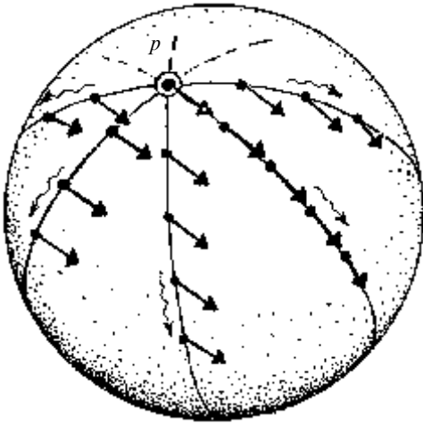
Fig. 14.3 Parallel transport of \mathbf{v} along five different paths (all great circles).
