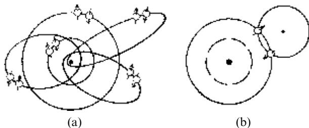
Fig. 24.2 Evidence of electron's spin \frac{1}{2} . (a) In an atom, two electrons, but not more, can occupy the same orbital. This is achieved by their spin states being opposite, so the Pauli exclusion principle is not violated. (b) Chemistry's 'covalent bond' involves a pair of electrons of opposite spin sharing orbitals of two separate atoms.
