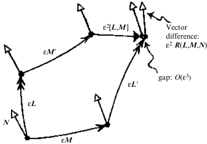
Fig. 14.19 Curvature, in the ‘mathematician’s notation’ (\nabla_L M - \nabla_M L - \nabla_{[M, L]} N) = R(L, M, N) , from the O(\epsilon^2) discrepancy in parallel transport of a vector N around the (incomplete) ‘quadrilateral’ with sides \epsilon L , \epsilon M , \epsilon L' , \epsilon M' . The Lie bracket contribution \epsilon^2[L, M] fills an O(\epsilon^2) gap, to order O(\epsilon^3) . (The index form of the vector R(L, M, N) is L^a M^b N^c R_{abc}{}^d .)
