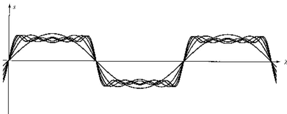
Fig. 9.12 Partial sums of the Fourier series s(\chi) = \sin \chi + \frac{1}{3} \sin 3\chi + \frac{1}{5} \sin 5\chi + \frac{1}{7} \sin 7\chi + \frac{1}{9} \sin 9\chi + \dots , converging to a square wave (like that of Fig. 9.11a).
