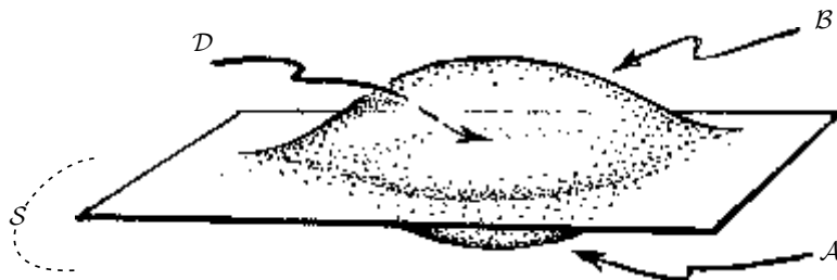
Fig. 20.9 Hamilton's principle for field Lagrangians. The two fixed end-points a , b , in \mathcal{C} , of Fig. 20.3, represent field configurations in two 3-dimensional spacetime regions \mathcal{A} , \mathcal{B} , respectively—forming a ‘blister’ which encloses the 4-region \mathcal{D} . We may take \mathcal{A} and \mathcal{B} to come together, terminating at a finite 2-surface S (not drawn in the figure), or we may regard ‘ S ’ to be out at infinity, perhaps out along a spacelike hypersurface throughout which \mathcal{A} and \mathcal{B} coincide beyond the region \mathcal{D} (the case illustrated).
