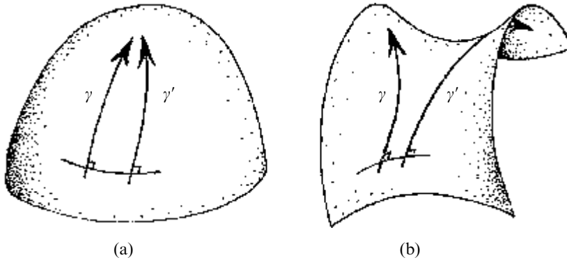
Fig. 14.12 Geodesic deviation when \mathcal{M} is a 2-surface (a) of positive (Gaussian) curvature, when the geodesics \gamma , \gamma' bend towards each other, and (b) of negative curvature, when they bend apart.
