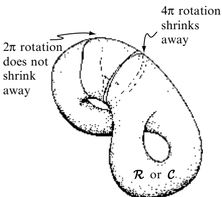
Fig. 12.3 The notion of multiple connectivity, as illustrated in Fig. 12.2, distinguishes the topology of the 3-manifold \mathcal{R} (rotation space), or of the 6-manifold \mathcal{C} (configuration space), from the ‘trivial’ topologies of Euclidean 3-space and 6-space. A loop on \mathcal{R} or \mathcal{C} representing a continuous rotation through 2\pi cannot be shrunk to a point, so \mathcal{R} and \mathcal{C} are multiply-connected. Yet, when traversed twice (representing a 4\pi -rotation) the loop does shrink to a point (topological torsion). See Fig. 11.3. (N.B. The 2-manifold depicted, being schematic only, does not actually have this last property.)
