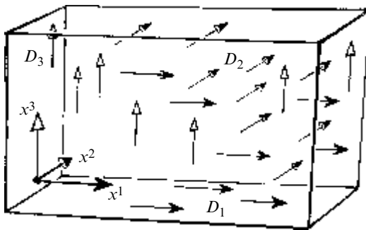
Fig. 21.1 In (affine) Euclidean N -space \mathbb{E}^N , there are N independent translational symmetries generated by the operators (vector fields)
