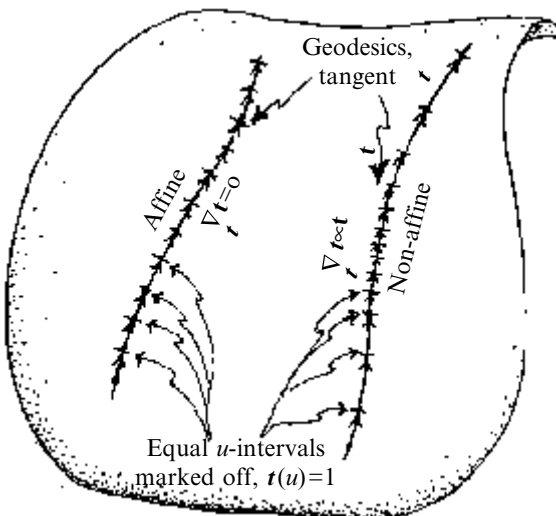
Fig. 14.8 For any (suitably smooth) parameter u defined along a curve \gamma , a field of tangent vectors \mathbf{t} to \gamma is naturally associated with u so that, along \gamma , \mathbf{t} stands for d/du (equivalently \mathbf{t}(u) = 1 , or t^a \nabla_a u = 1 ). If \gamma is a geodesic, u is called an affine parameter if \mathbf{t} is parallel-transported along \gamma , so \nabla_{\mathbf{t}} \mathbf{t} = 0 rather than just \nabla_{\mathbf{t}} \mathbf{t} \propto \mathbf{t} . An affine parameter is ‘evenly spaced’ along \gamma , according to \nabla .
