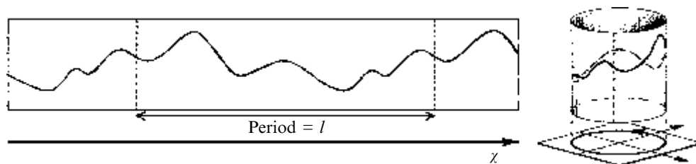
Fig. 9.3 A periodic function of a real variable \chi may be thought of as defined on a circle of circumference l where we ‘wrap up’ the real axis of \chi into the circle. With l = 2\pi , we may take this circle as the unit circle in the complex plane.
