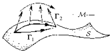
Fig. 32.2 We can express \Gamma = \Gamma_1 + i\Gamma_2 , where \Gamma_1 refers to the intrinsic curvature and \Gamma_2 to the extrinsic curvature of S (so \Gamma_2 measures how S ‘bends’ within \mathcal{M} ).
