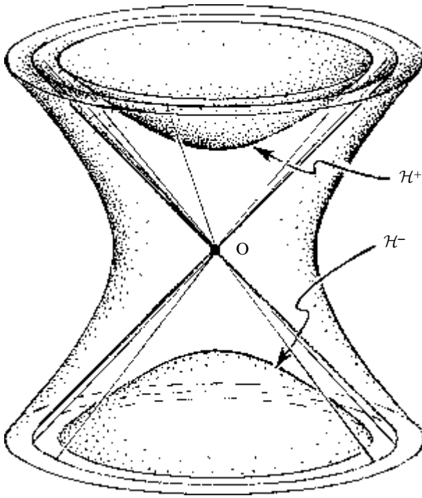
Fig. 18.7 ‘Spheres’ in \mathbb{M} , as the loci of points a fixed Minkowski distance a from a fixed point O .
