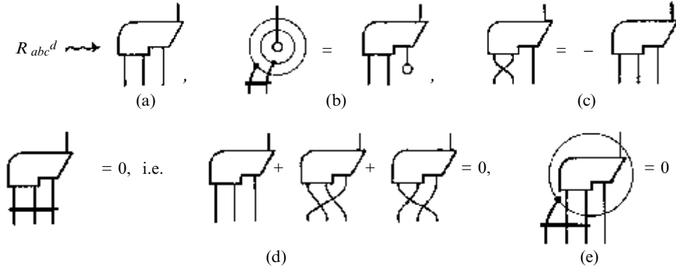
Fig. 14.7 (a) A convenient diagrammatic notation for the curvature tensor R_{abc}{}^d . (b) The Ricci identity (\nabla_a \nabla_b - \nabla_b \nabla_a)\xi^d = R_{abc}{}^d \xi^c . (c) The antisymmetry R_{bac}{}^d = -R_{abc}{}^d . (d) The Bianchi symmetry R_{[abc]}{}^d = 0 , which reduces to R_{abc}{}^d + R_{bca}{}^d + R_{cab}{}^d = 0 . (e) The Bianchi identity \nabla_{[a} R_{bc]d}{}^e = 0 .
