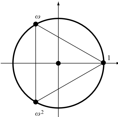
Fig. 5.11 Equilateral triangle of cube roots 1, \omega , and \omega^2 of unity. Multiplication by \omega rotates through 120^\circ anticlockwise, and by \omega^2 , clockwise.
