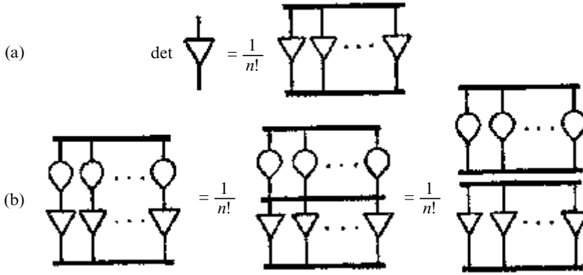
Fig. 13.8 (a) Diagrammatic notation for \det (T^a_b) = \det \mathbf{T} = |\mathbf{T}| . (b) Diagrammatic proof that \det (\mathbf{ST}) = \det \mathbf{S} \det \mathbf{T} . The antisymmetrizing bar can be inserted in the middle term because there is already antisymmetry in the index lines that it crosses. See Figs. 12.17, 12.18.
