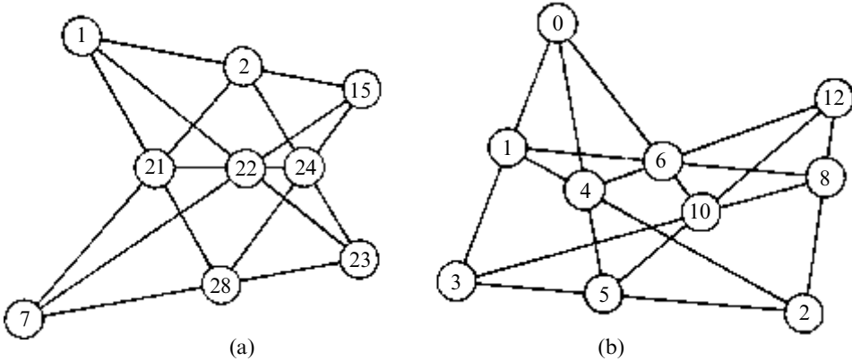
Fig. 16.2 Finite-geometry versions of the theorems of Fig. 5.14. (a) Pappos (with q=5 ) and (b) Desargues (with q=3 ), illustrated by respective use of the discs shown in Fig. 16.1d and 16.1b.
