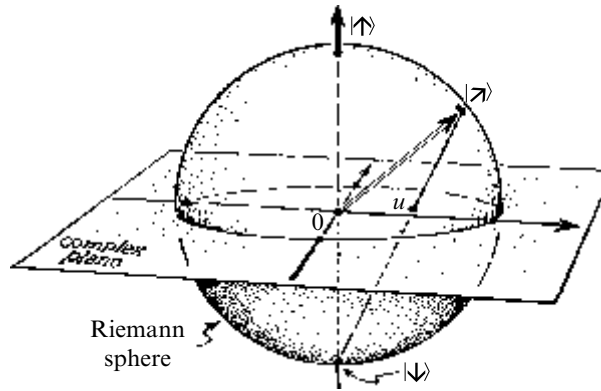
Fig. 22.10 The projective space \mathbb{P}\mathbf{H}^2 for 2-state system is a Riemann sphere (see Fig. 8.9). For the spin states of a massive particle of spin \frac{1}{2} , we can use the north pole to represent the spin state |\uparrow\rangle (spin ‘up’) and the south pole, the state |\downarrow\rangle (spin ‘down’). A general spin state |\nearrow\rangle is represented (with appropriate phases for |\uparrow\rangle and |\downarrow\rangle ) by the point on the sphere whose direction out from the centre is that of |\nearrow\rangle (i.e. which gives the result ‘YES’ with certainty for a spin measurement E_{\nearrow} in that direction), as illustrated by the double-shafted arrow. We can express the state |\nearrow\rangle as a linear combination |\nearrow\rangle = w|\uparrow\rangle + z|\downarrow\rangle (where we can regard the complex numbers z, w as the components w = \psi_0, z = \psi_1 of a 2-spinor \psi_A ). The points on the sphere correspond to the distinct ratios z:w . Each of these can be represented by a complex number u = z/w (allowing \infty ) in the complex plane, this plane being taken to be the equatorial plane of the sphere. The point u projects stereographically from the south pole to the point on the sphere representing |\nearrow\rangle .
