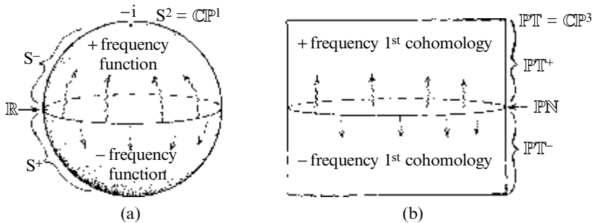
Fig. 33.22 An analogy between the Riemann sphere S^2 (= \mathbb{C}P^1) and projective twistor space \mathbb{P}T (= \mathbb{C}P^3) . (a) A complex function (i.e. a ‘0th cohomology element’), defined on the real axis \mathbb{R} of S^2 , splits into its positive frequency part, extending holomorphically into what is here depicted as the northern hemisphere S^- , and its negative frequency part, extending into the southern hemisphere S^+ . (The Riemann sphere is here drawn so that \mathbb{R} is its equator, but so that -i is at the north pole and i at the south pole; compare Figs. 8.7 and 9.10, §9.5.) (b) A 1st cohomology element, defined on \mathbb{P}N (and representing a massless field) splits into its positive frequency part, extending holomorphically into the top half \mathbb{P}T^+ of projective twistor space, and its negative frequency part, extending into the bottom half \mathbb{P}T^- .
