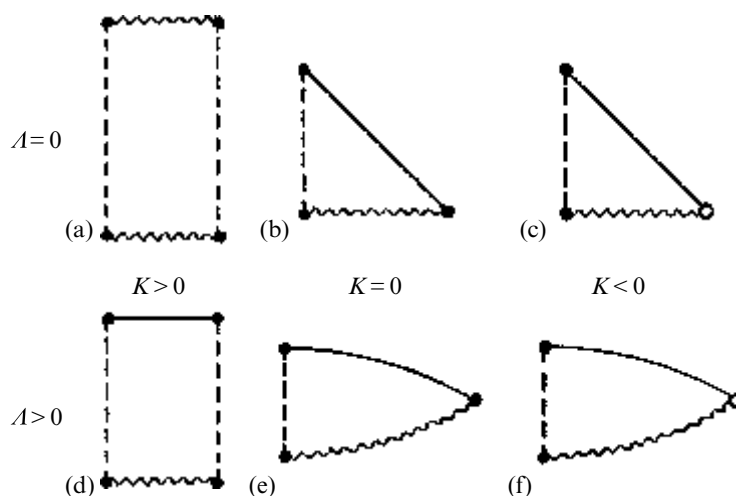
Fig. 27.17 Strict conformal diagrams for the respective Friedmann models of Fig. 27.13: (a) K > 0 , \Lambda = 0 ; (b) K = 0 , \Lambda = 0 ; (c) K < 0 , \Lambda = 0 ; (d) K > 0 , \Lambda > 0 (and \Lambda large enough); (e) K = 0 , \Lambda > 0 ; (f) K < 0 , \Lambda > 0 .
