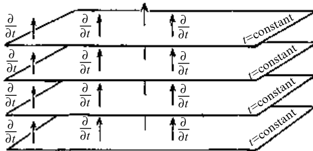
Fig. 30.22 Knowing t does not tell us \partial/\partial t (‘second fundamental confusion of calculus’, see Fig. 10.7, §10.3); t tells us where the \mathbb{E}^3 -sections lie, but \partial/\partial t defines a family of curves cutting across this family of 3-surfaces.
