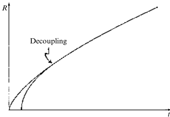
Fig. 27.14 Before ‘decoupling’, which occurred when the universe was about 300 000 years old (only about 1/50 000 of its present age)—the epoch we ‘look back’ to with the microwave background—the universe was ‘radiation dominated’ and Friedmann’s ‘dust’ approximation did not hold. Instead, we have the somewhat more rapid Tolman expansion, indicated by the inner curve.
