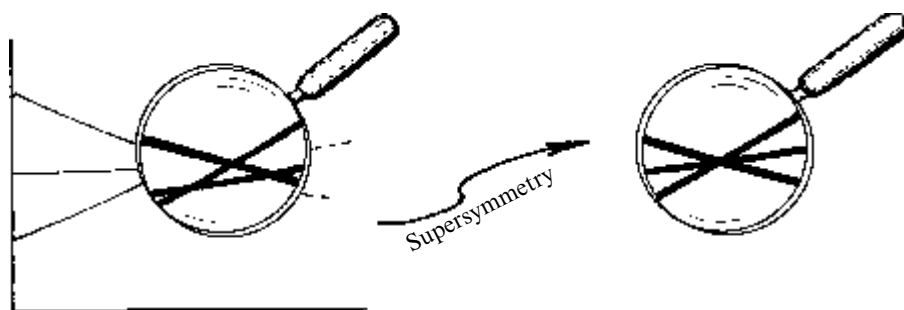
Fig. 31.1 According to a certain ‘grand-unified’ perspective, the coupling constants of strong, weak, and electromagnetic interactions, treated as ‘running coupling constants’ (see Note 26.21 and §31.1), should all attain exactly the same value at large enough temperatures, about 10^{28} K, which would have occurred at around 10 000 Planck moments after the Big Bang ( \sim 10^{-39} s). It was found that supersymmetry is needed in order to bring all three values precisely together.
