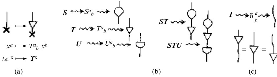
Fig. 13.6 (a) The linear transformation x^a \mapsto T^a_b x^b , or written without indices as x \mapsto T^x (or read with the indices as abstract, as in §12.8), in diagrammatic form. (b) Diagrams for linear transformations S , T , U , and their products ST and STU . In a successive product, we string them in a line downwards. (c) The Kronecker delta \delta^a_b , or identity transformation I , is depicted as a ‘disembodied’ line, so relations T^a_b \delta^b_c = T^a_c = \delta^a_b T^b_c become automatic in the notation (see also Fig. 12.17).
