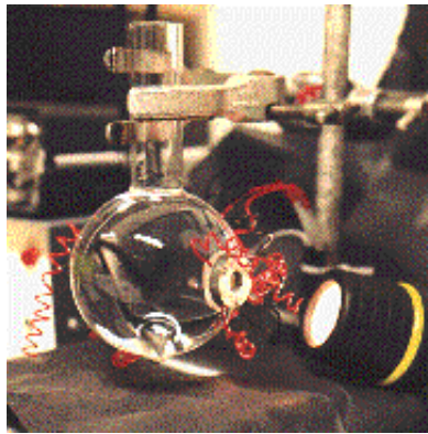
Sonoluminescence experiment
