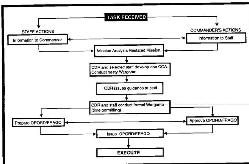
Figure 3-1. Accelerated MDMP.
