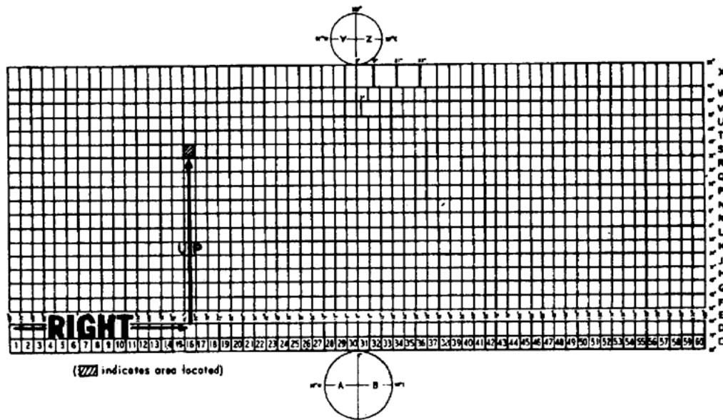
Figure 4-8. UTM grid zone location.
