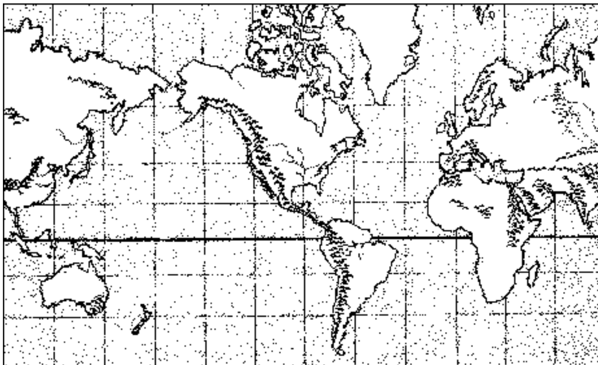
Figure 13-2. Mountain systems.
