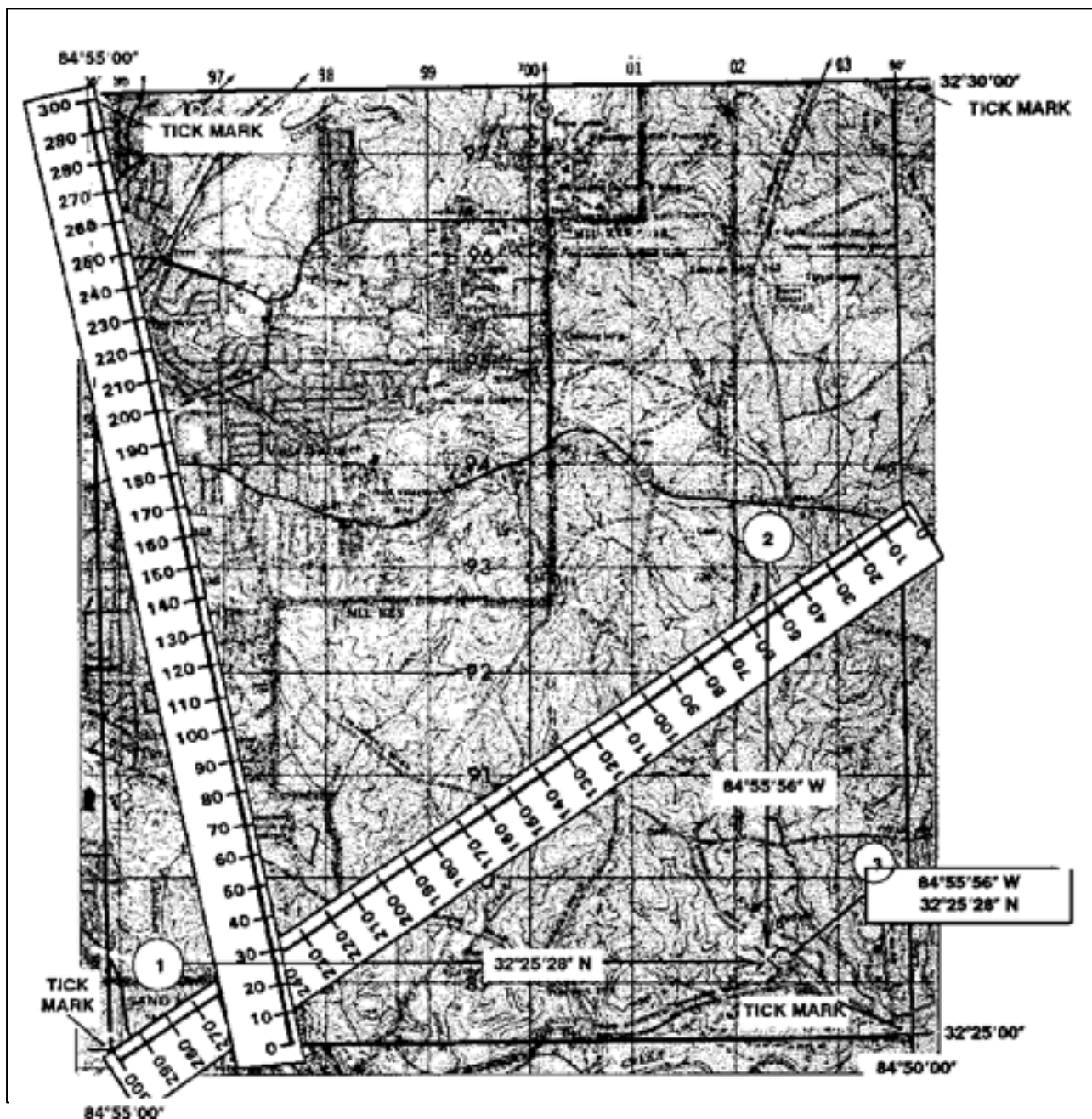
Figure 4-6. Determining geographic coordinates.
