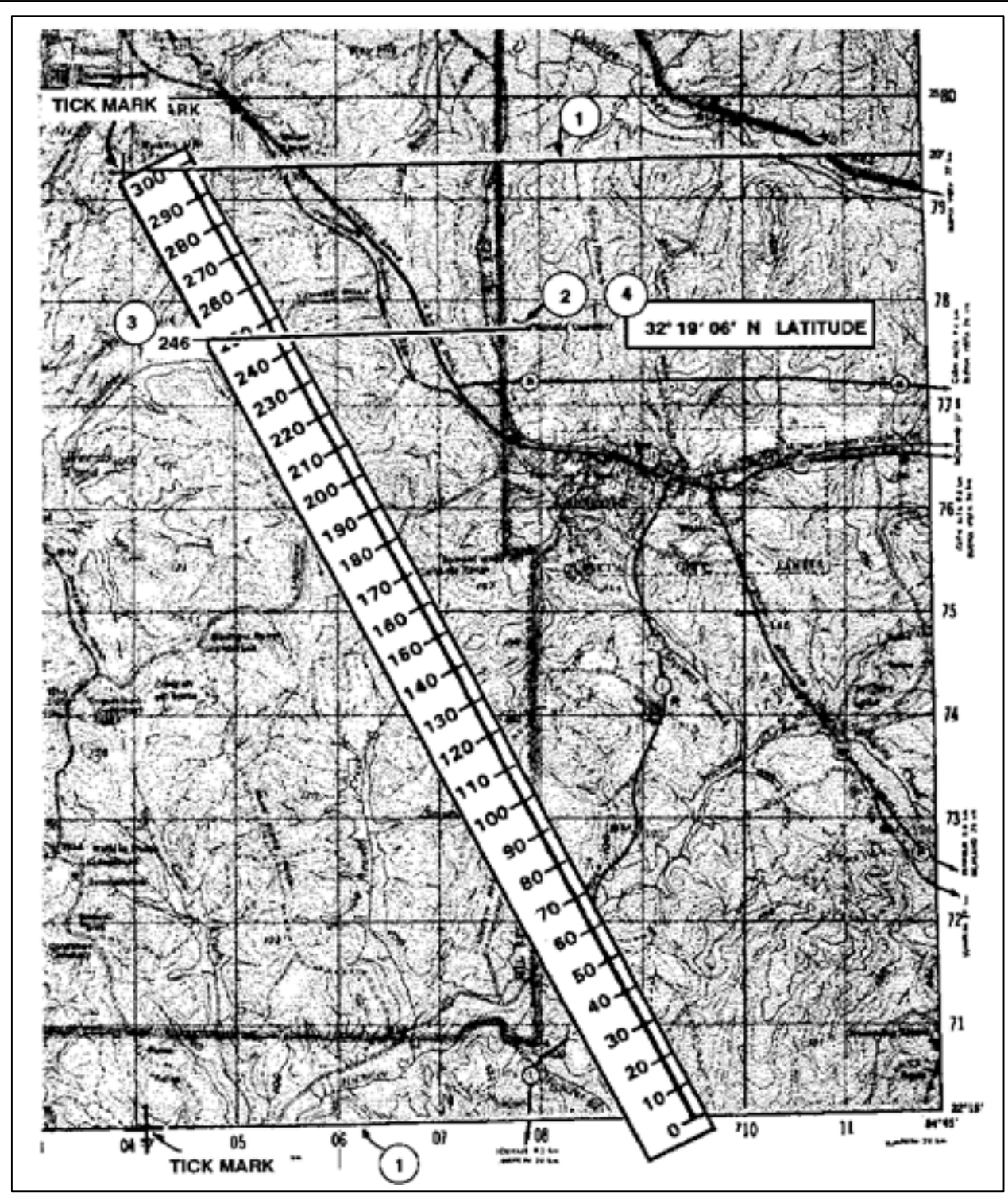
Figure 4-4. Determining latitude.
