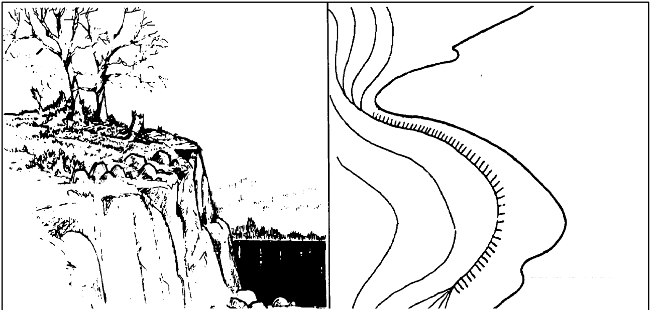
Figure 10-24A. Cliff.
