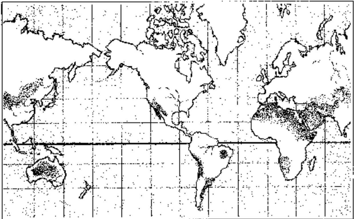
Figure 13-1 Deserts.
