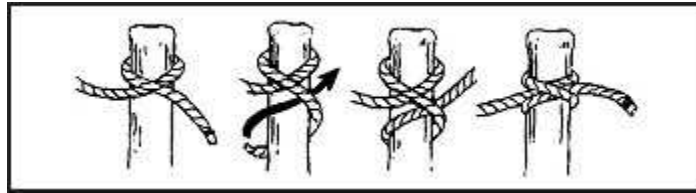
Figure G-6. End-of-the-Line Clove Hitch
