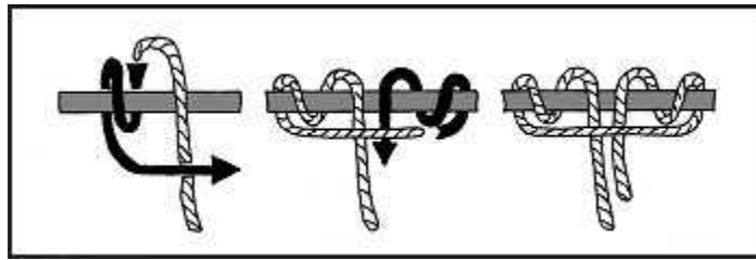
Figure G-9. Prusik, End of Line
