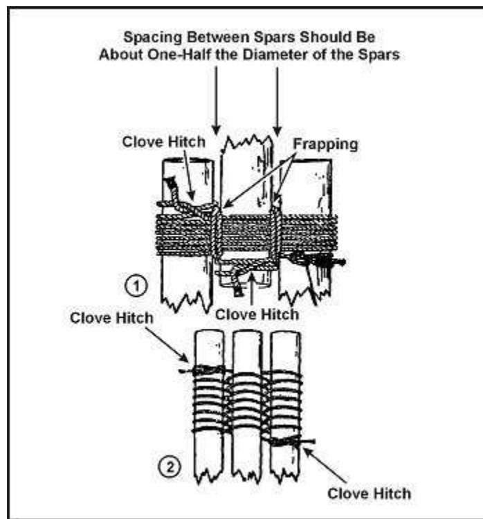
Figure G-16. Tripod Lashing
