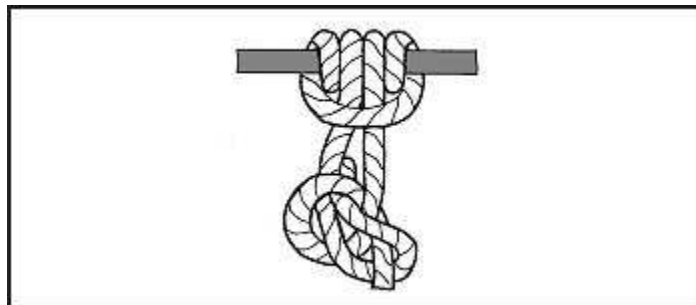
Figure G-11. Prusik, End of Line With Bowline for Safety
