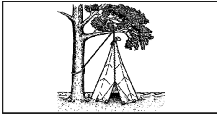
Figure 5-6. No-Pole Parachute Tepee
