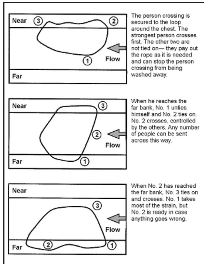
Figure 17-3. Individuals Tied Together to Cross Stream
