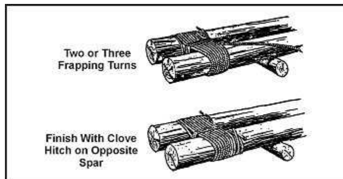
Figure G-14. Shears Lashing
