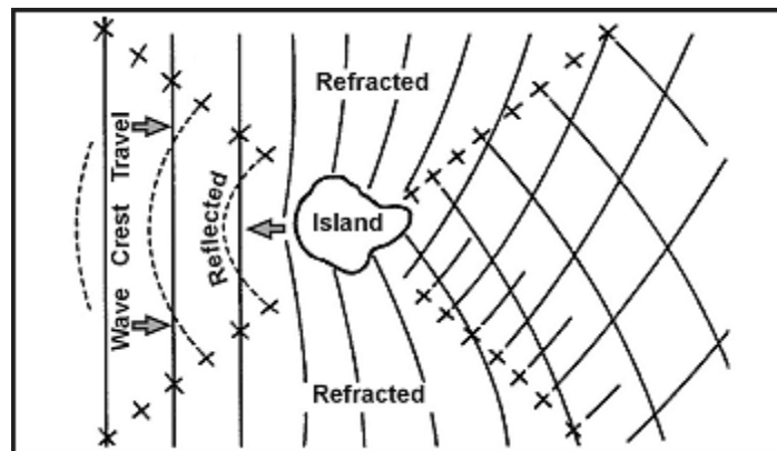
Figure 16-18. Wave Patterns About an Island
