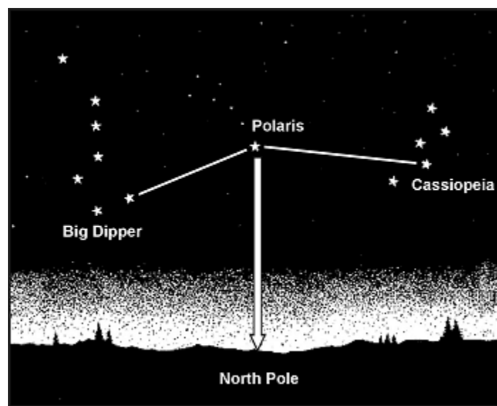
Figure 18-3. The Big Dipper and Cassiopeia
