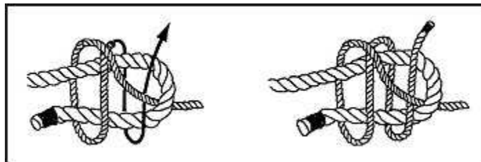
Figure G-8. Double Sheet Bend
