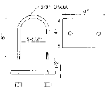
U-BOLT & BEARING PLATE
