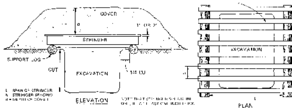
Figure B-1 DESIGN PROCEDURE DATA Soil Parameters
