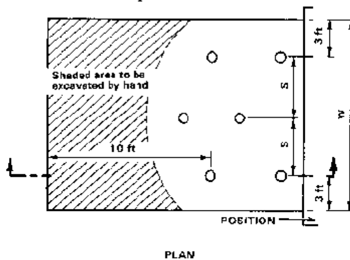
Boreholes for positions in flat terrain
