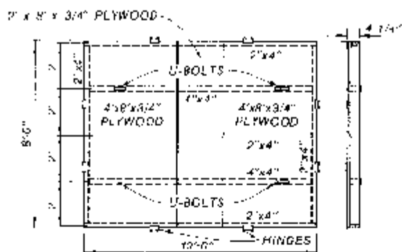
FLOOR DETAIL
