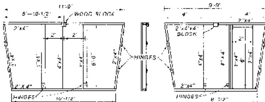
SIDE WALL DETAIL
