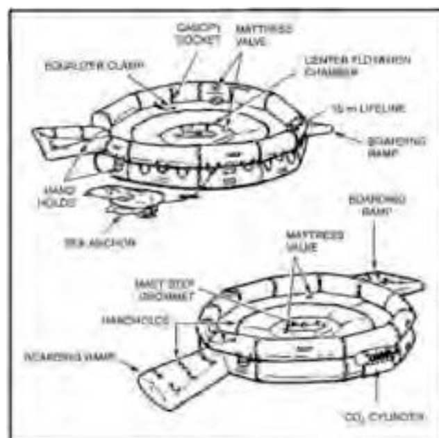
Figure 16-15. Two-man raft.
