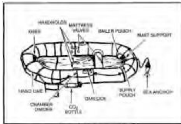
Figure 16-12. Navy-style raft.
