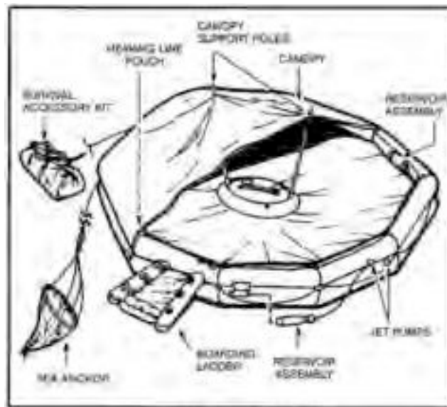
Figure 16-16. Group/Breast raft.
