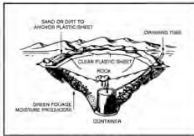
Figure 8-3. Atmowood still.
