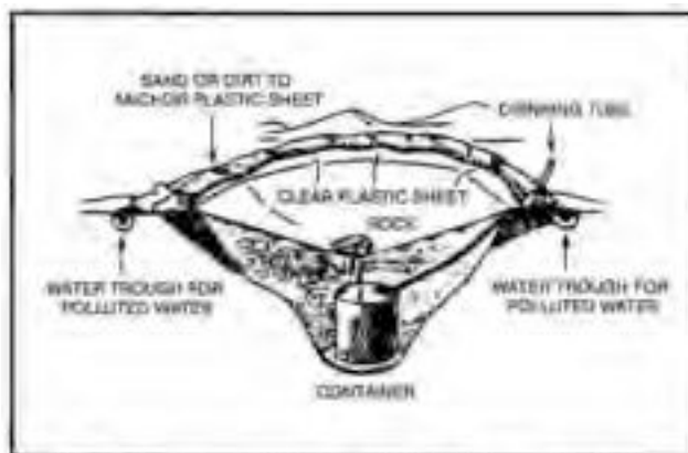
Figure 6-8. Retain ground still to get potable water from polluted water.
