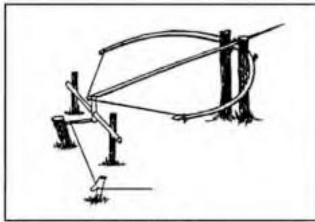
Figure 8-14. Bow trap.
