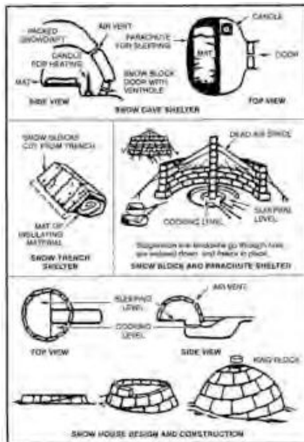
Figure 15-4. Snow shelters.
