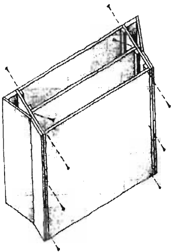
Figure 7-5a. Volume displacement box (VDB) for forming window opening. Illustration from The Rammed Earth House by David Easton (Chelsea Green Publishing Company, 1996).
