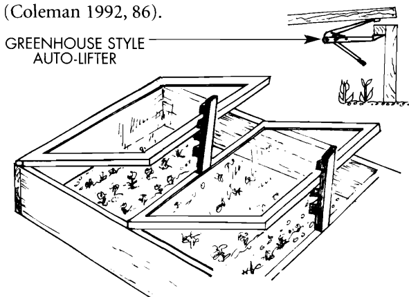
Figure 6-14. Cold frames.
