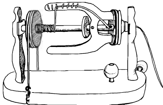
Figure 10-8. Spinning wheel flyer and bobbin.
