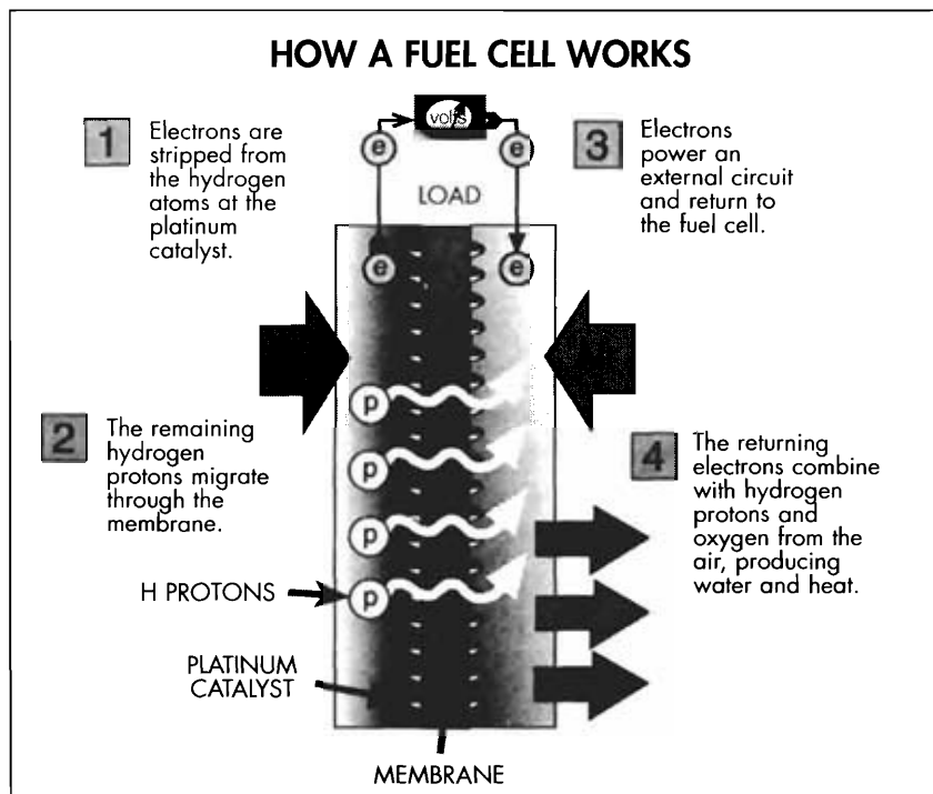
Figure 11-13. How a fuel cell works. Illustration courtesy of Home Power Magazine .
