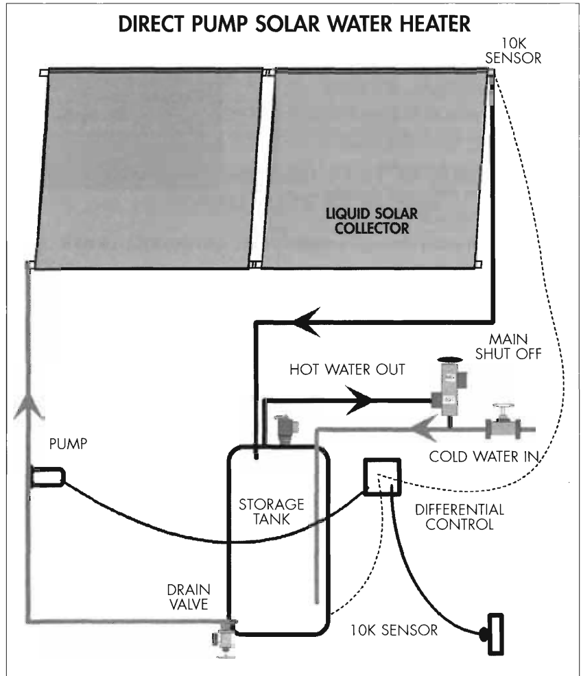
Figure 11-8. Direct pump type solar water heater. Illustration courtesy of AAA Solar.
