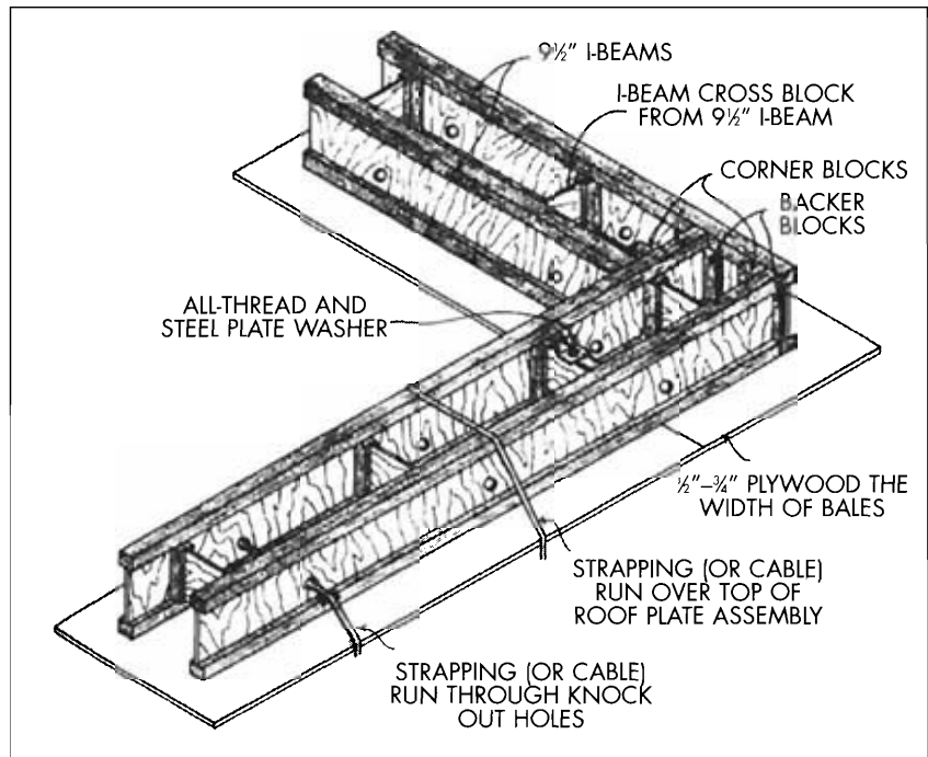
Figure 7-12. Bond beam for load-bearing walls, showing strapping and all-thread options. Illustration from The Straw Bale House by Athena Swentzell Steen, Bill Steen, and David Brainbridge with David Eisenberg (Chelsea Green Publishing Company, 1994).
