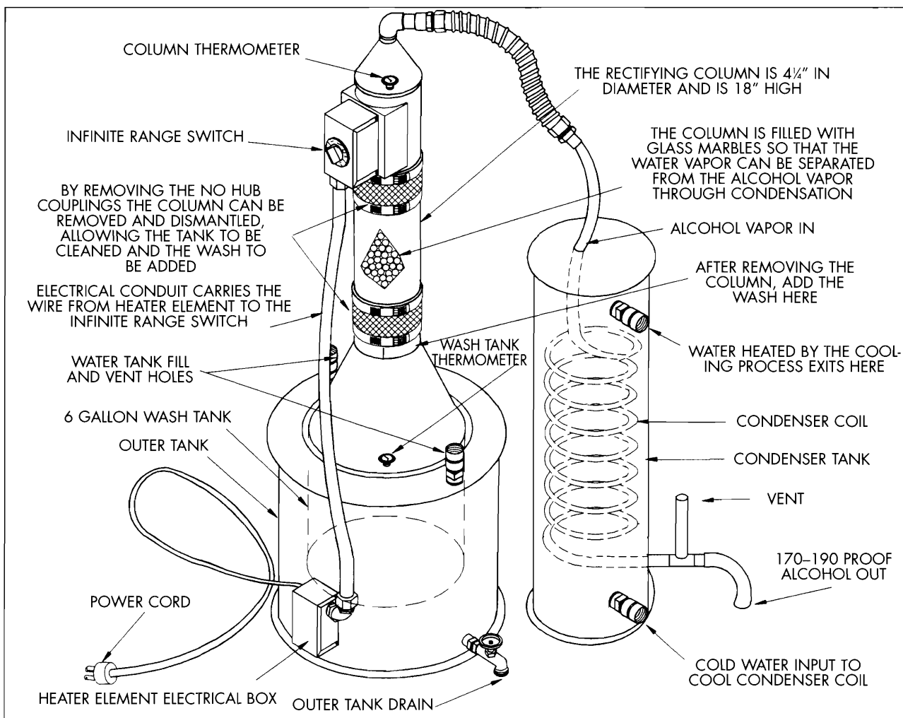
Figure 14-7. Vince Gingery's homemade electric still. Illustration courtesy of The Secrets of Building an Alcohol-Producing Still by Vincent R. Gingery (David J. Gingery Publishing, 1994).
