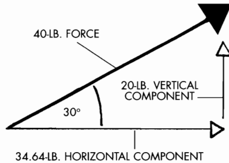
Figure 15-2. Components of a force.
