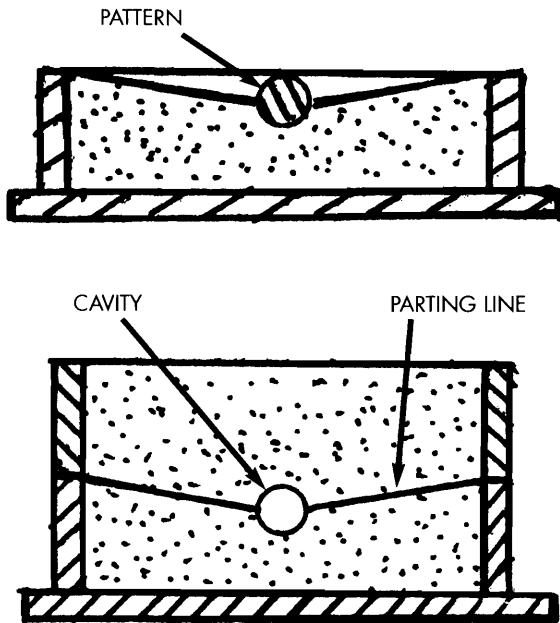
Figure 12-5. “Coping down” to match the parting line. Illustration courtesy of The Charcoal Foundry by David J. Gingery [Gingery, 1983].
