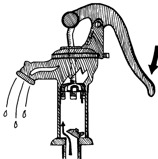
Figure 5-8b. Shallow well hand pump, output stroke.
