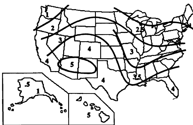
Figure 11-3. December/January average equivalent sun hours per day. Illustration courtesy of Sierra Solar Systems.
