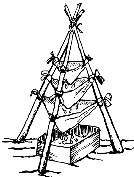
Figure 5-2. Crude sand filter.
