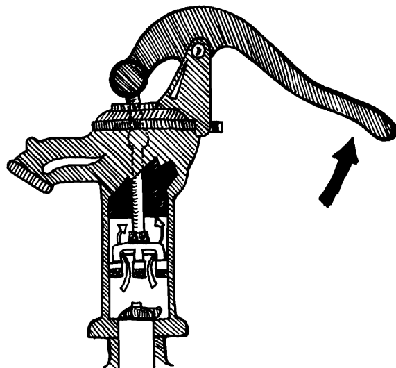
Figure 5-8a. Shallow well hand pump, intake stroke.
