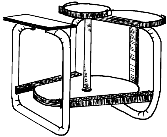
Figure 13-18. Low-tech kick wheel.
