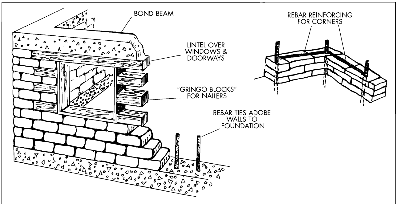
Figure 7-8. Typical adobe wall construction.
