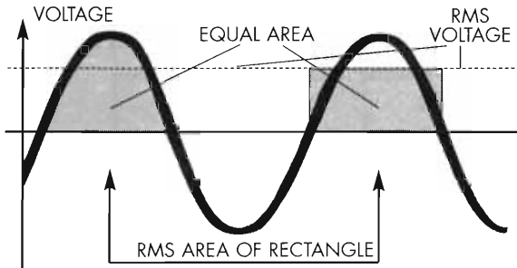
Figure 11-19. Sinusoidal alternating current (AC).
