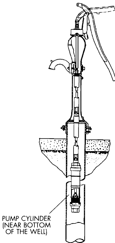
Figure 5-9. Deep well hand pump. Illustration courtesy of Baker Manufacturing Company, Monitor Division.
