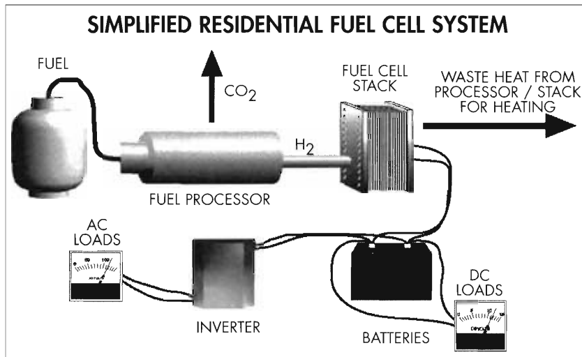
Figure 11-14. Simplified residential fuel cell system. Illustration courtesy of Home Power Magazine .
