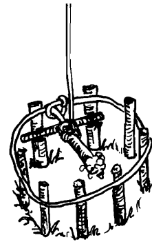
Figure 6-44. T-bar snare.
