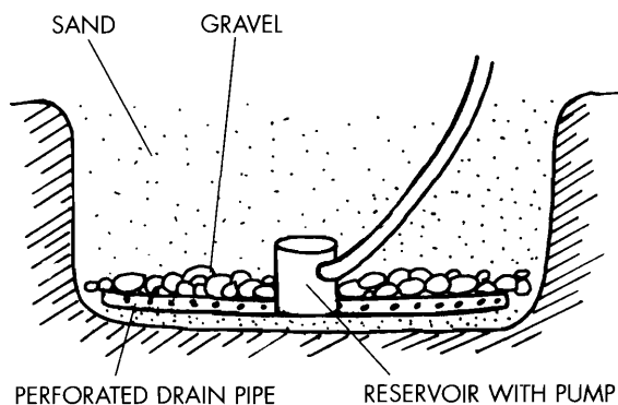
Figure 5-1. Slow sand filter reservoir.
