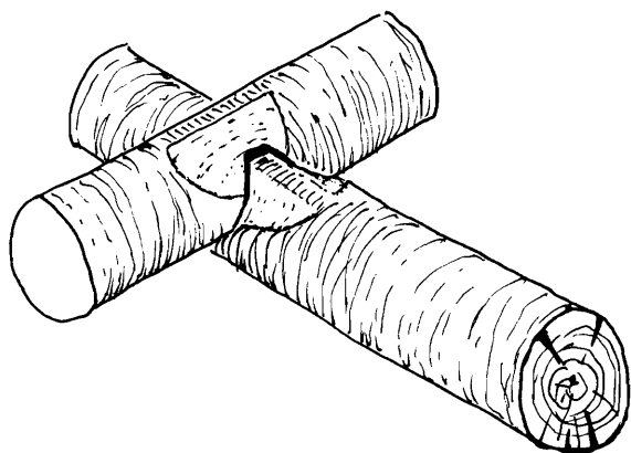
Figure 7-17. Common modern log notch and saddle. Illustration adapted from Log Building Construction Manual by Robert Chambers (1999).
