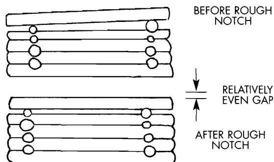
Figure 7-19. Rough notch, then scribe for "scribe-fit" log groove. Illustrations adapted from Log Building Construction Manual by Robert Chambers (1999).
