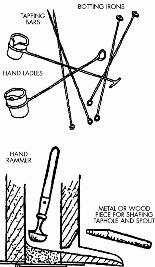
Figure 12-8. Tools for making up the bottom and operating the cupola. Illustration courtesy of Building Small Cupola Furnaces by Stewart Marshall (1996).
