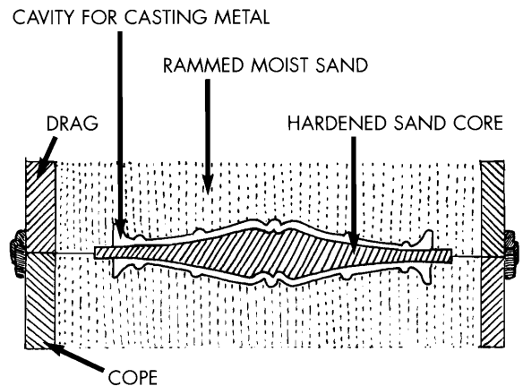
Figure 12-4. A sand mold with a baked sand core to cast a hollow column. Adapted from an illustration courtesy of Metalworking: A Book of Tools, Materials and Processes for the Handyman by Paul N. Hasluck (Lindsay Publications, 1994).
