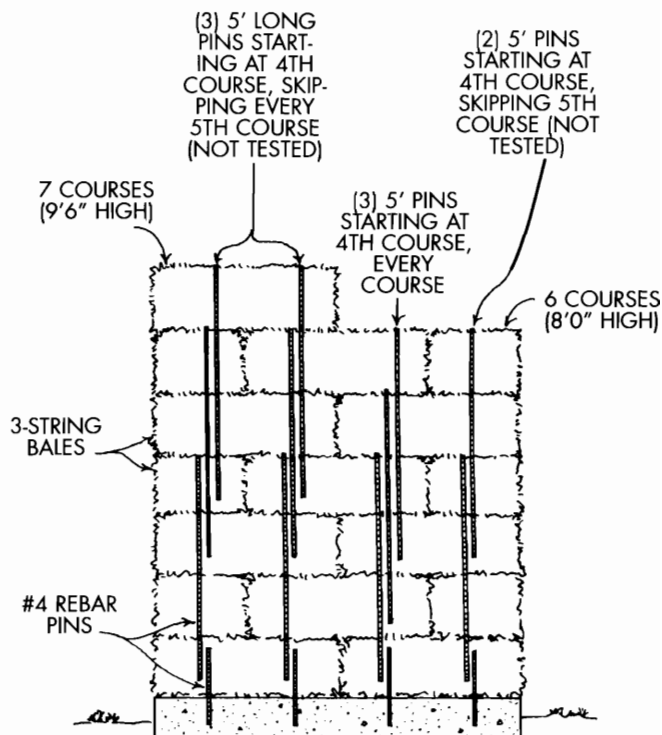
Figure 7-11. Bale-pinning options. Illustration from The Straw Bale House by Athena Swentzell Steen, Bill Steen, and David Brainbridge with David Eisenberg (Chelsea Green Publishing Company, 1994).
