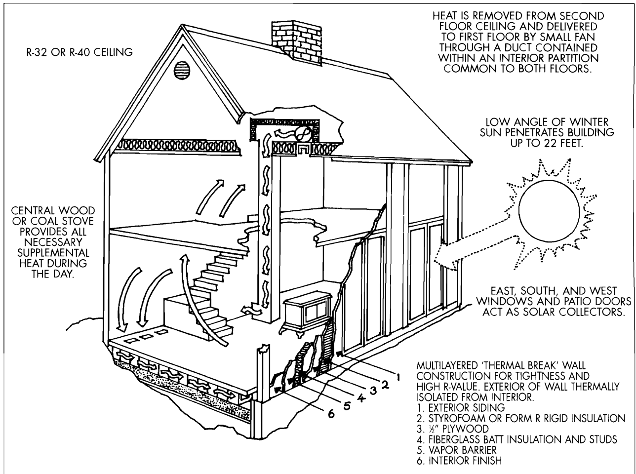
Figure 7-15. Heating a house with James Kachadorian's solar slab heat exchanger. Illustration courtesy of Chelsea Green Publishing Company (Kachadorian 1997).
