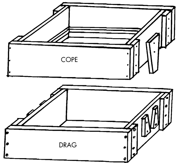
Figure 12-3. The casting flasks. Illustration courtesy of The Charcoal Foundry by David J. Gingery (Gingery, 1983).
