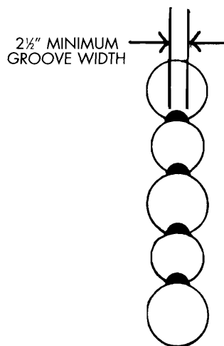
Figure 7-16. Custom-cut grooves to fit log rows to each other. Illustration adapted from Log Building Construction Manual by Robert Chambers (1999).
