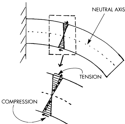
Figure 15-6. Beam bending.
