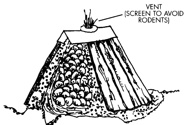
Figure 6-36a. Aboveground storage: vented "mound."
