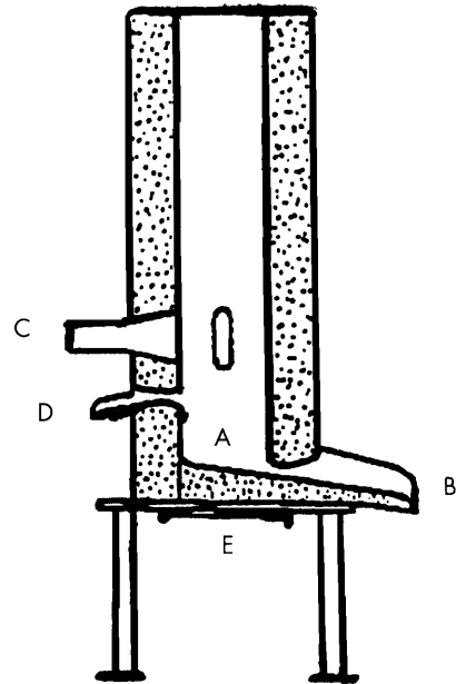
Figure 12-6. Basic construction of a small cupolette. Illustration courtesy of Building Small Cupola Furnaces by Stewart Marshall (1996).
