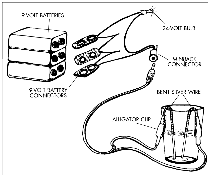
Figure 9-1. Colloidal silver generator.
