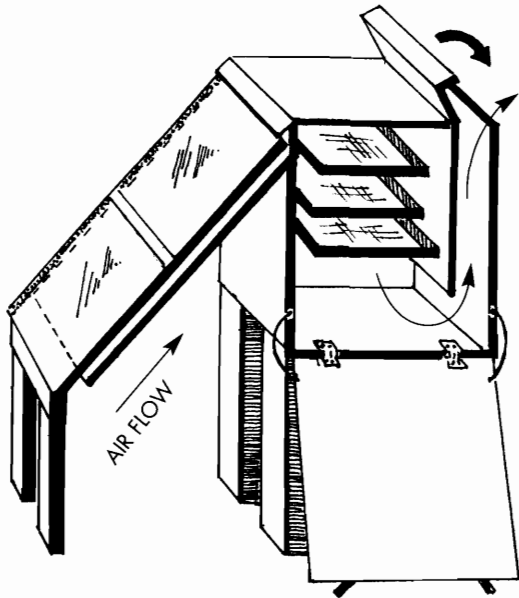
Figure 6-37. Solar dryer.
