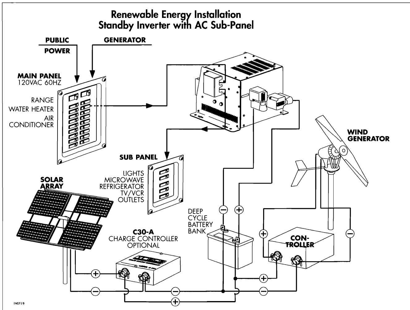
Figure 11-1. Typical renewable energy system with a multifunction inverter. Illustration courtesy of Trace Engineering.
