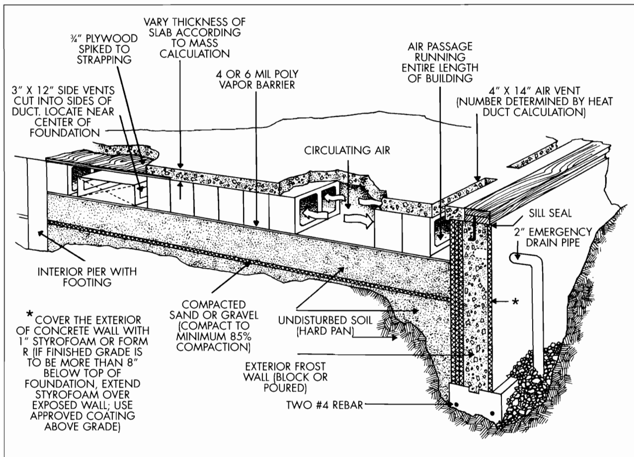
Figure 7-14. James Kachadorian's solar slab heat exchanger detail. Illustration courtesy of Chelsea Green Publishing Company (Kachadorian 1997).
