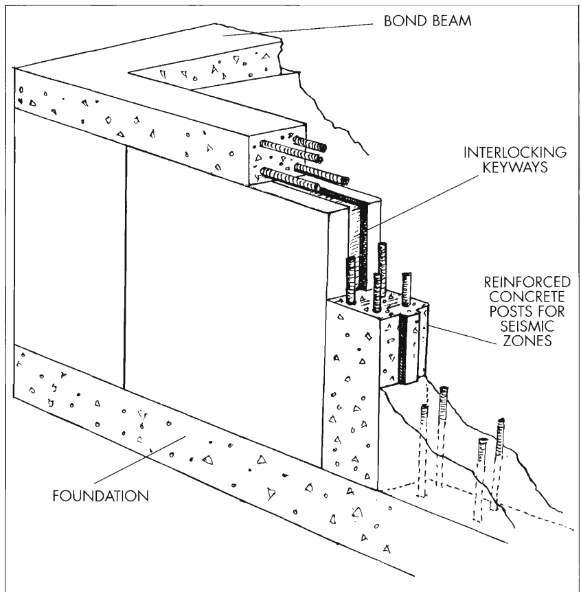
Figure 7-4. Rammed earth wall section (note interlocking keyways).
