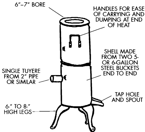
Figure 12-7. Small portable cupolette furnace for iron castings up to 10 lbs. or bronze to 20 lbs. Illustration courtesy of Building Small Cupola Furnaces by Stewart Marshall (1996).
