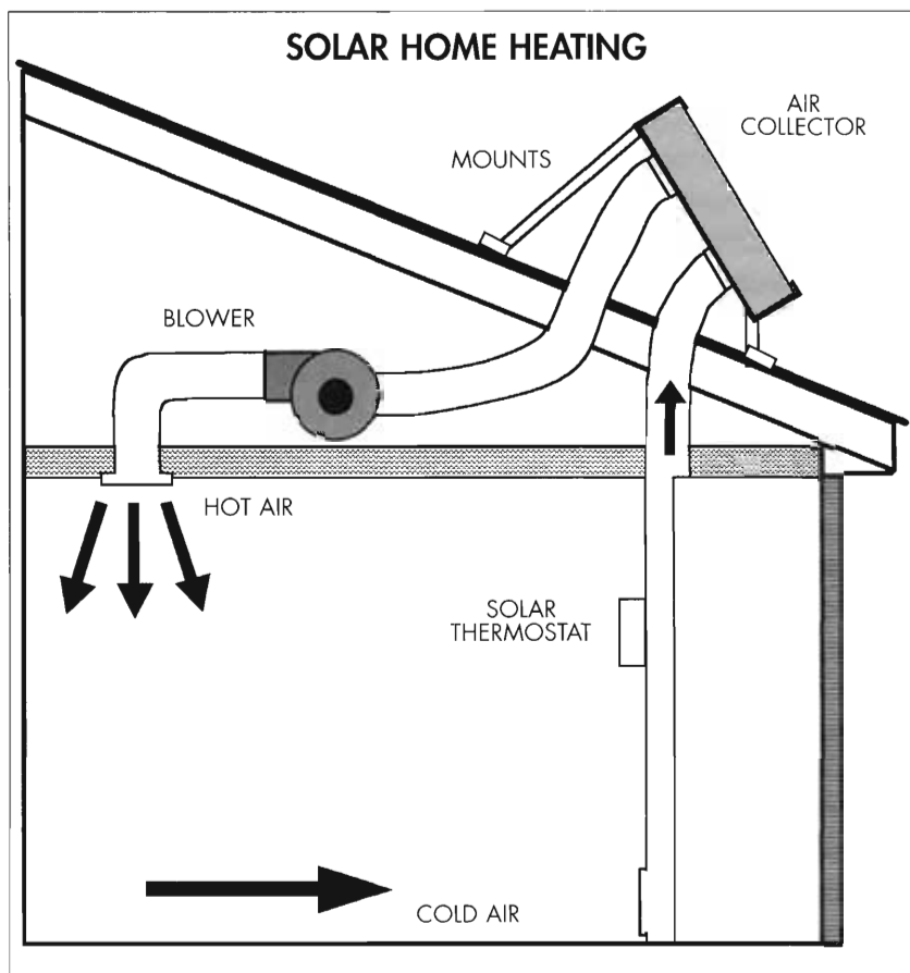
Figure 11-10. Active solar space heating with hot air solar collectors. Illustration courtesy of AAA Solar.
