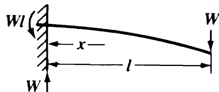
Figure 15-10. Diagram for case 3. Illustration courtesy of Machinery's Handbook , 26th ed., edited by Erik Oberg, Franklin D. Jones, Holbrook L. Horton, Henry H. Ryffel, and Christopher J. McCauley (Industrial Press, 2000).
