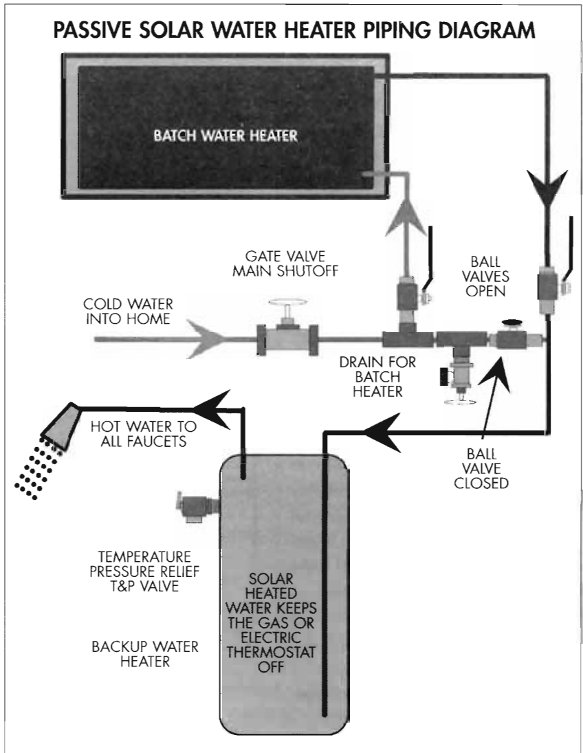
Figure 11-7. Solar batch water heater. Illustration courtesy of AAA Solar.
