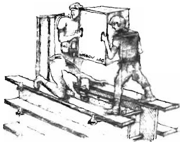
Figure 7-5b. Placement of volume displacement box (VDB) for forming window opening. Illustration from The Rammed Earth House by David Easton (Chelsea Green Publishing Company, 1996).
