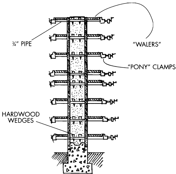
Figure 7-2. David Easton's rammed earth works forms. Adapted from an illustration from The Rammed Earth House by David Easton (Chelsea Green Publishing Company, 1996).
