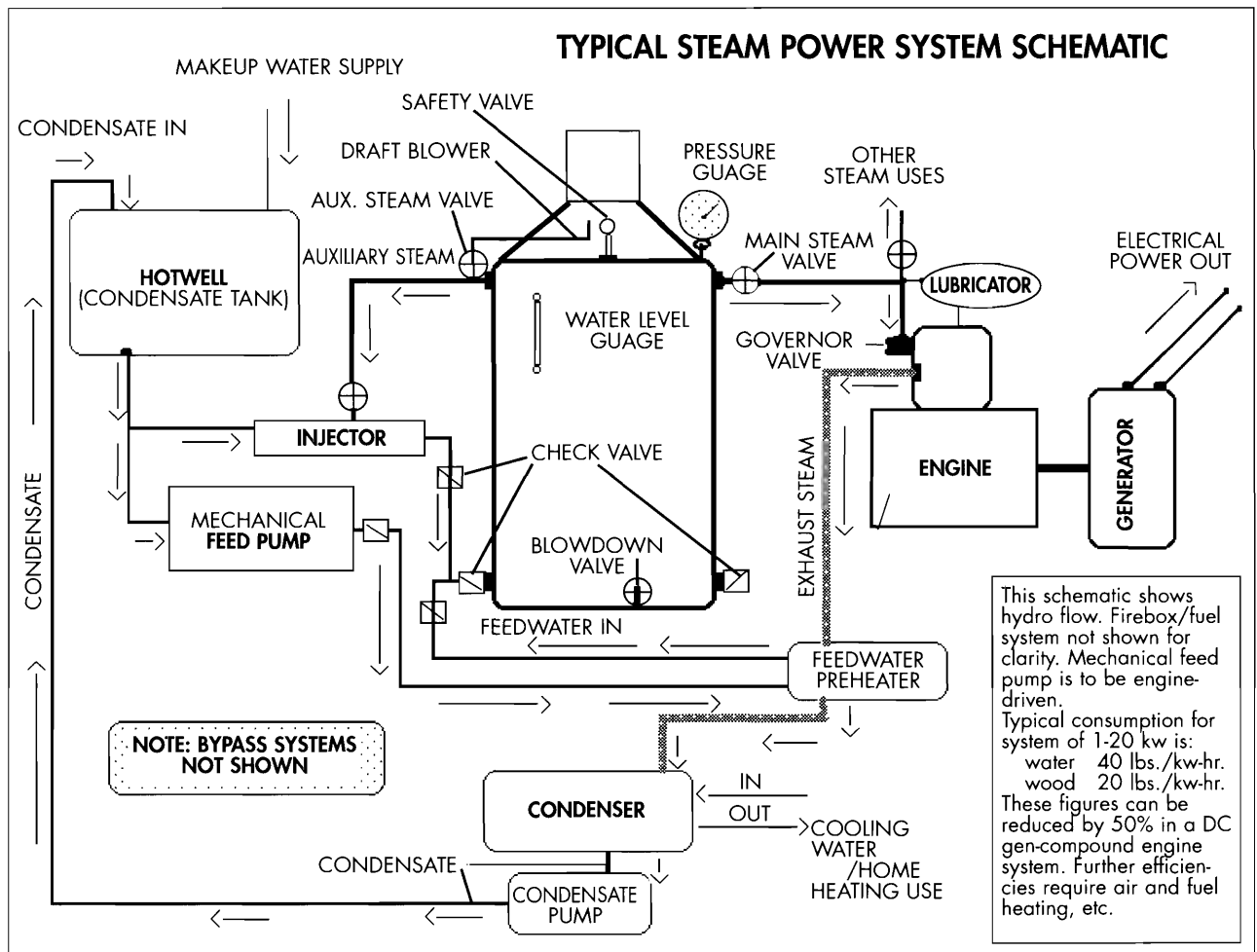
Figure 11-12. Steam-powered electricity generation. Illustration courtesy of Sensible Steam Consultants.
