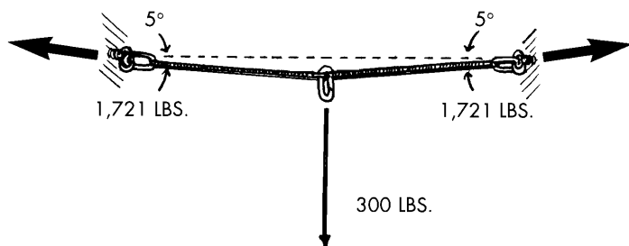
Figure 15-3. "Free body diagram" for two 150-pound rock climbers hanging on a couple of anchors.
