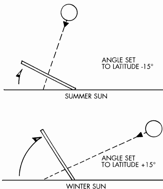
Figure 11-4. Panel seasonal orientation.
