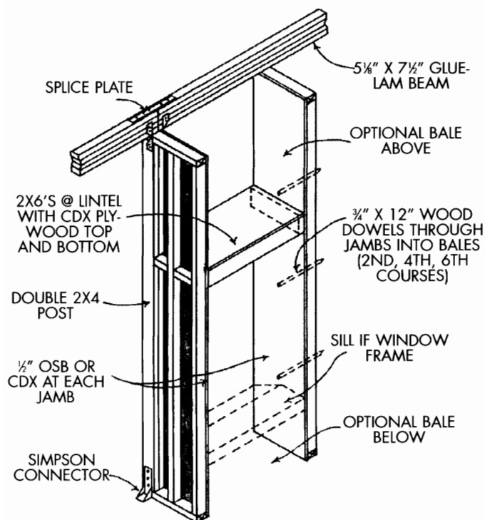
Figure 7-10. Box column detail for modified post-and-beam. Illustration from The Straw Bale House by Athena Swentzell Steen, Bill Steen, and David Brainbridge with David Eisenberg (Chelsea Green Publishing Company, 1994).
