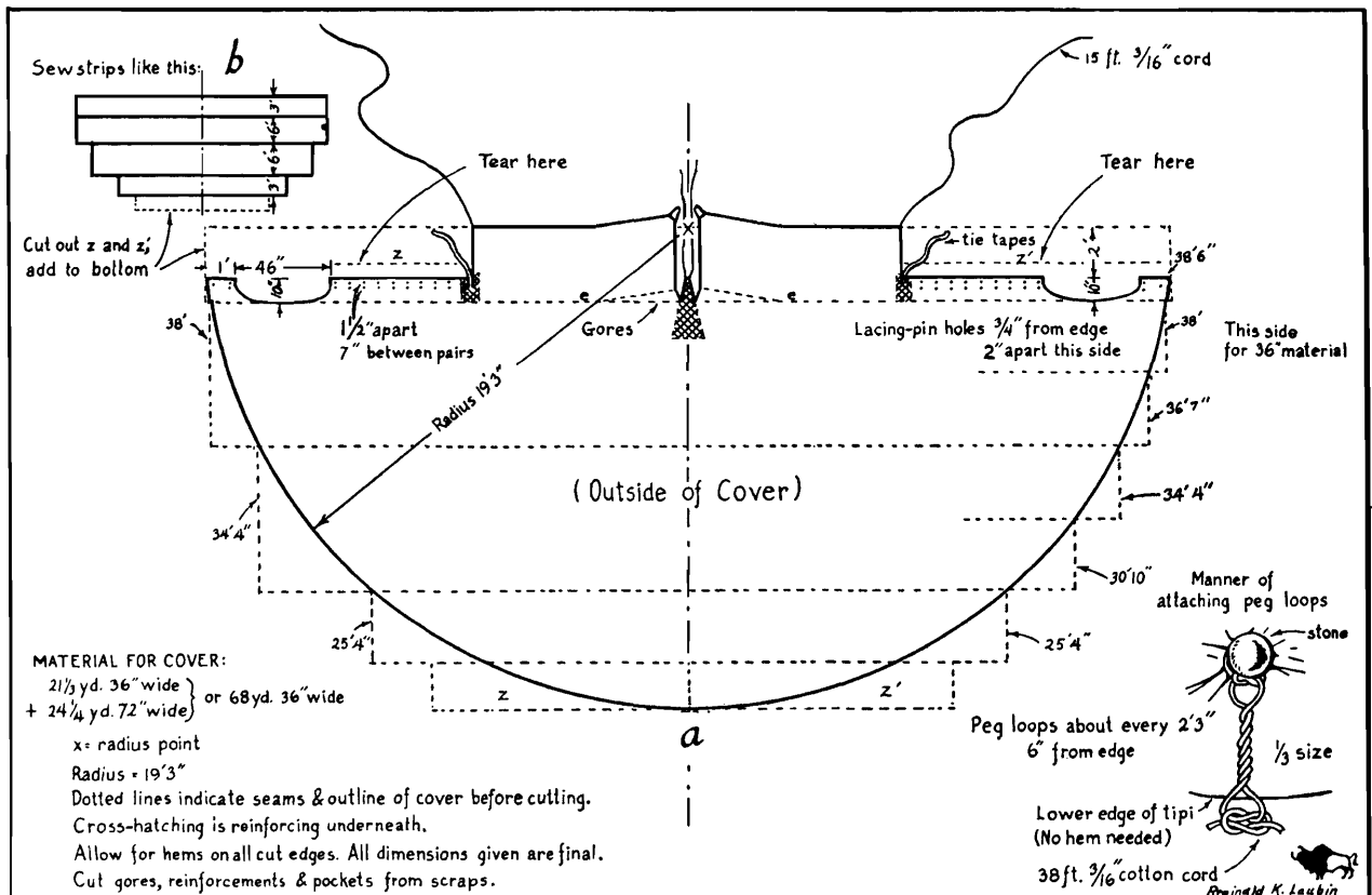
Figure 7-21. Basic 18-foot Sioux tipi pattern. Illustration from The Indian Tipi: Its History, Construction, and Use by Reginald Laubin and Gladys Laubin (University of Oklahoma Press, 1989).
