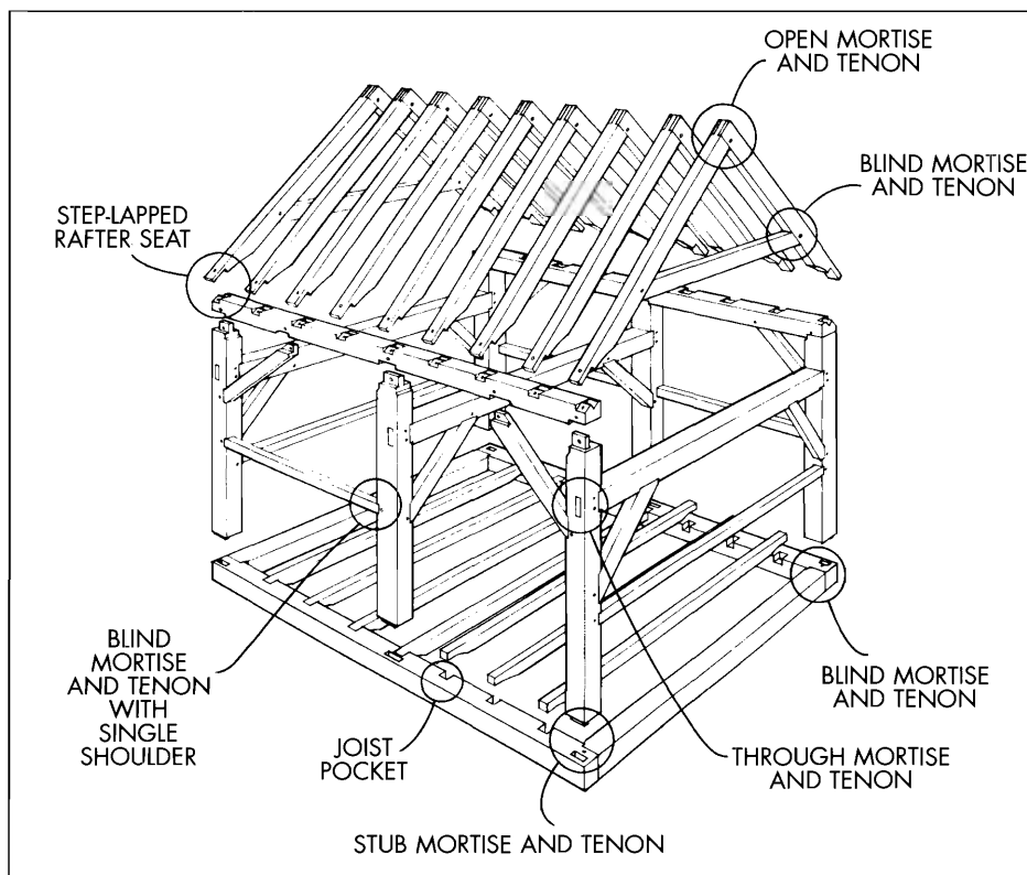
Figure 7-20. Simple timber frame showing several types of joints. Illustration from Timber Frame Construction: All About Post-and-Beam Building by Jack Sobon and Roger Schroeder (Storey Books 1984).
