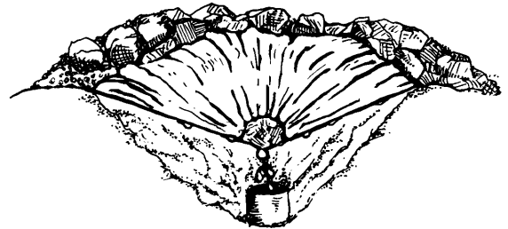
Figure 5-3. Solar still side view.
