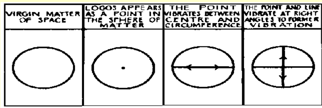
DIAGRAM III.—The Response of Matter.
