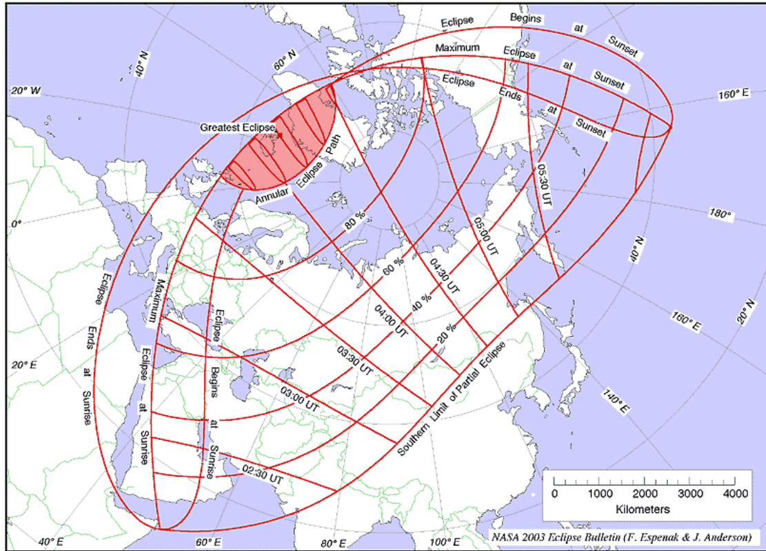
FIGURE 1.2 - STEREOGRAPHIC PROJECTION MAP OF THE ECLIPSE PATH
